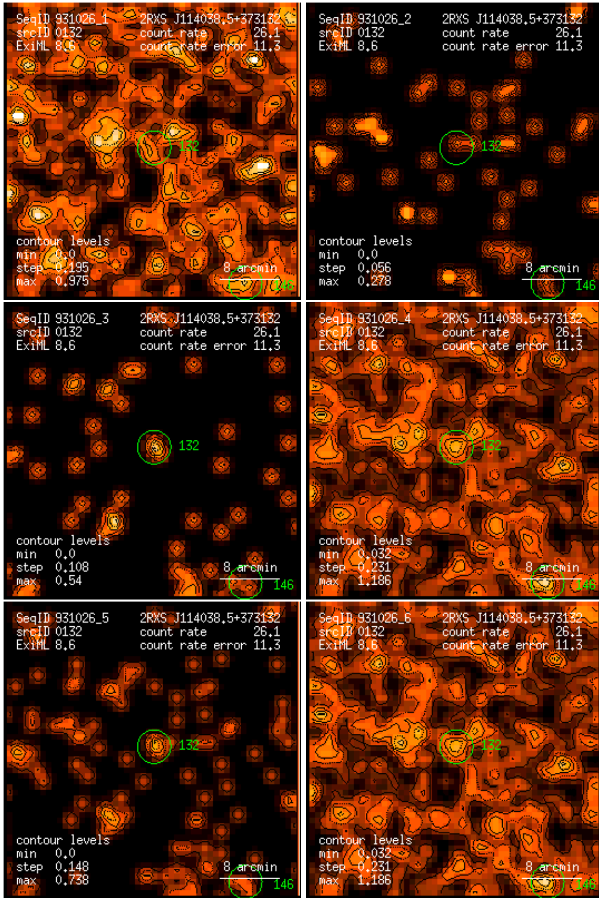
Figure 132: RASS 931026: detection 0132: band rate images, Gaussian filter: (1) PSPPC channels 11 – 41, (2) 52 – 90, (3) 91 – 201, (4) 11 – 235, (5) 52 – 201, (6) 11 – 201. Broad band rates in counts/ks. Band rate contour levels in counts/ks/arcmin 2 .
