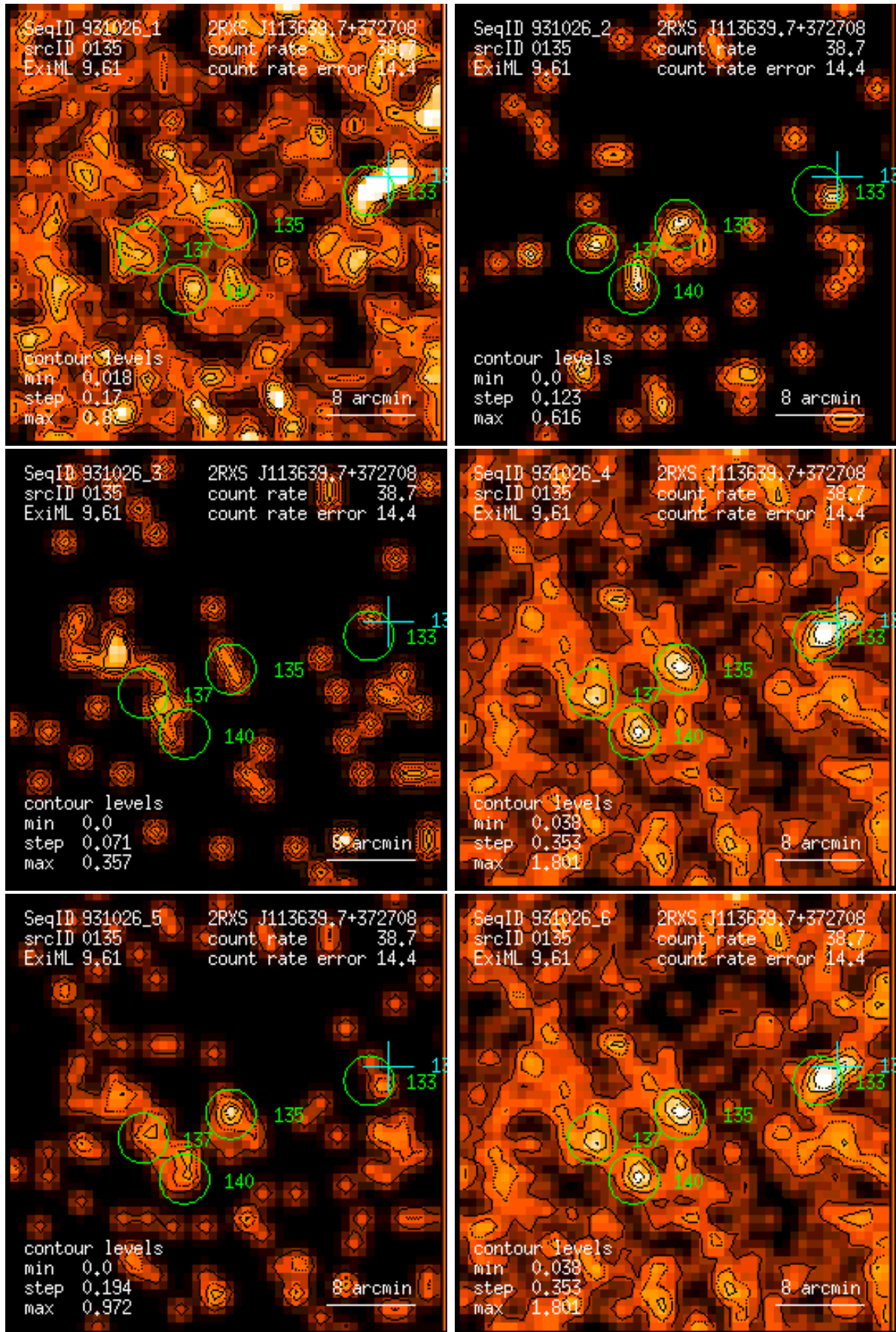
Figure 135: RASS 931026: detection 0135: band rate images, Gaussian filter: (1) PSPC channels 11 – 41, (2) 52 – 90, (3) 91 – 201, (4) 11 – 235, (5) 52 – 201, (6) 11 – 201. Broad band rates in counts/ks. Band rate contour levels in counts/ks/arcmin 2 .
