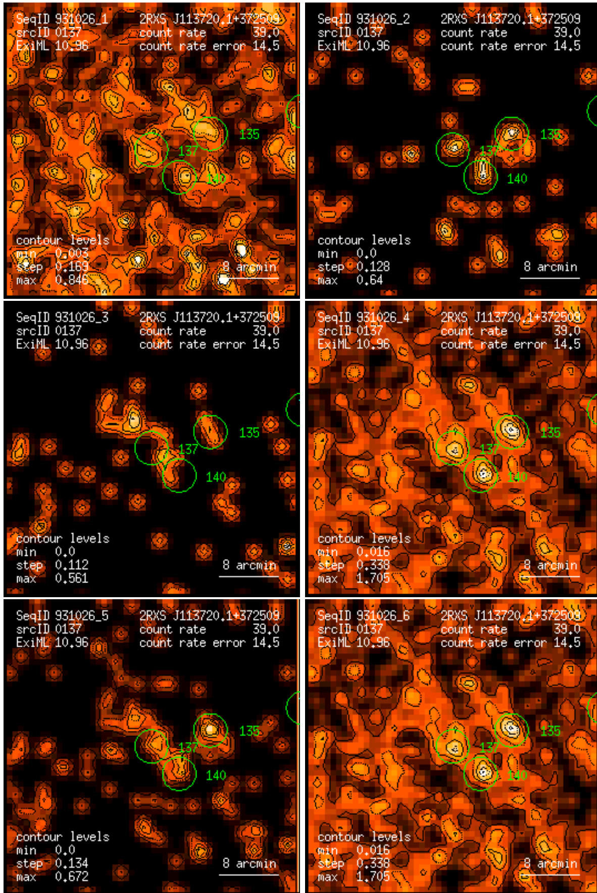
Figure 137: RASS 931026: detection 0137: band rate images, Gaussian filter: (1) PSPC channels 11 – 41, (2) 52 – 90, (3) 91 – 201, (4) 11 – 235, (5) 52 – 201, (6) 11 – 201. Broad band rates in counts/ks. Band rate contour levels in counts/ks/arcmin 2 .
