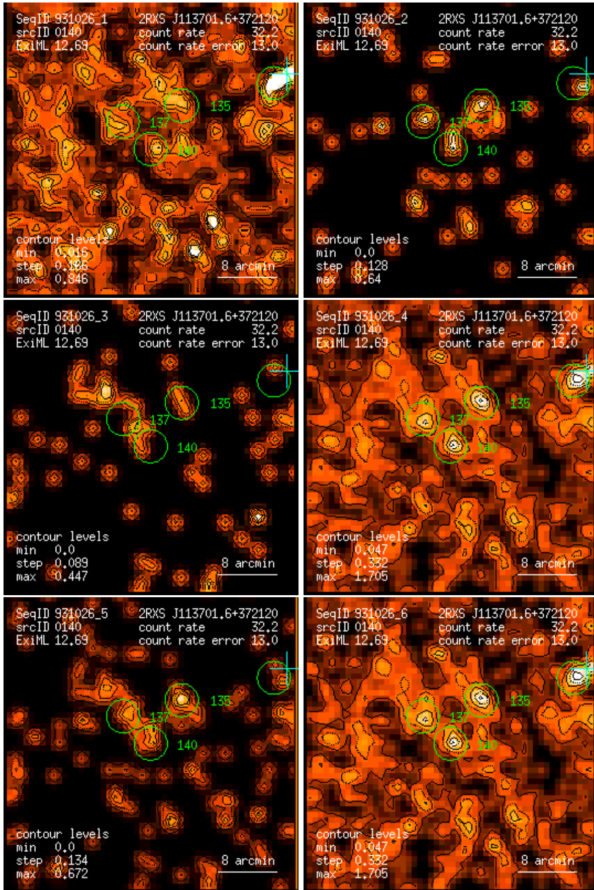
Figure 140: RASS 931026: detection 0140: band rate images, Gaussian filter: (1) PSPC channels 11 – 41, (2) 52 – 90, (3) 91 – 201, (4) 11 – 235, (5) 52 – 201, (6) 11 – 201. Broad band rates in counts/ks. Band rate contour levels in counts/ks/arcmin 2 .
