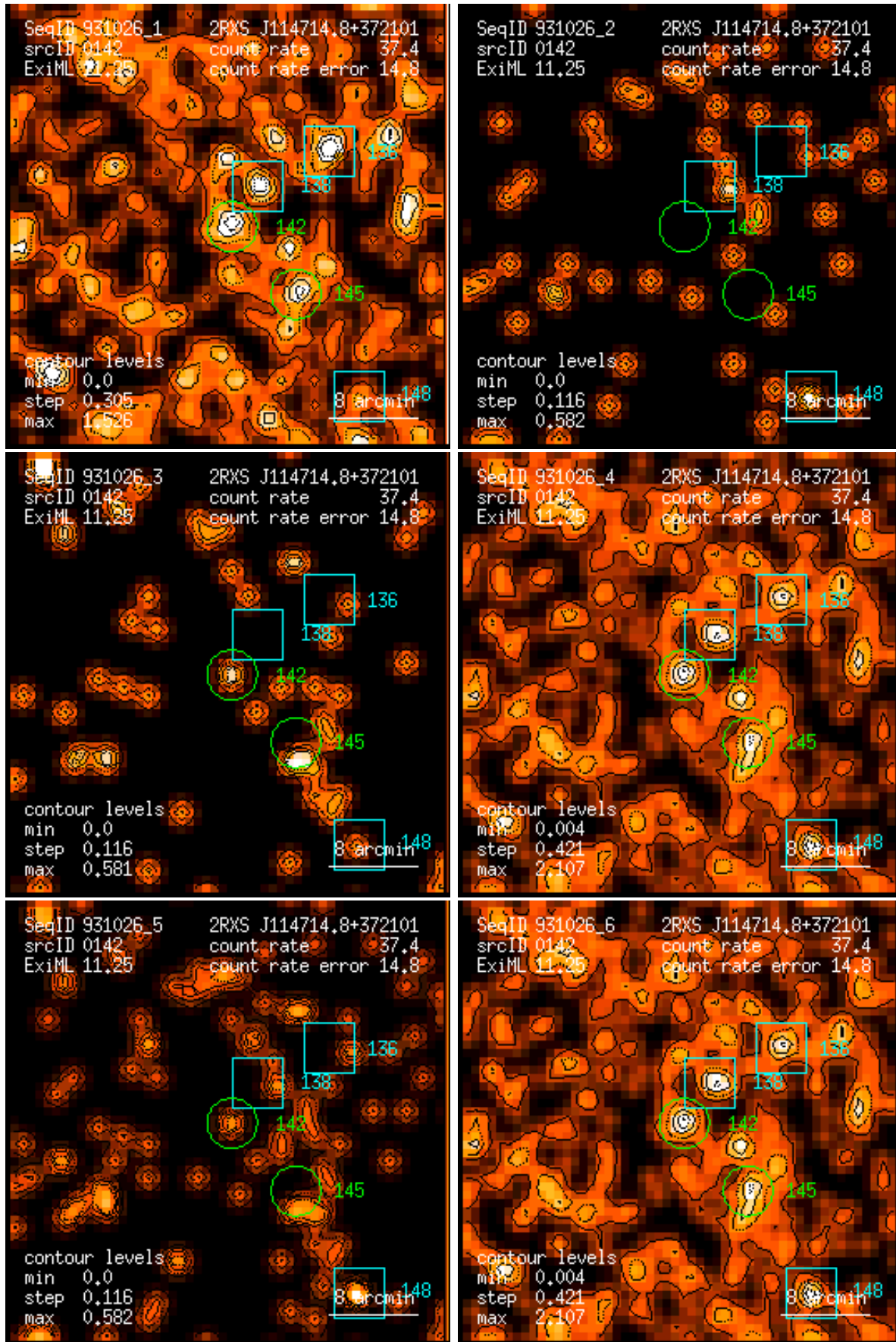
Figure 142: RASS 931026: detection 0142: band rate images, Gaussian filter: (1) PSPC channels 11 – 41, (2) 52 – 90, (3) 91 – 201, (4) 11 – 235, (5) 52 – 201, (6) 11 – 201. Broad band rates in counts/ks. Band rate contour levels in counts/ks/arcmin 2 .
