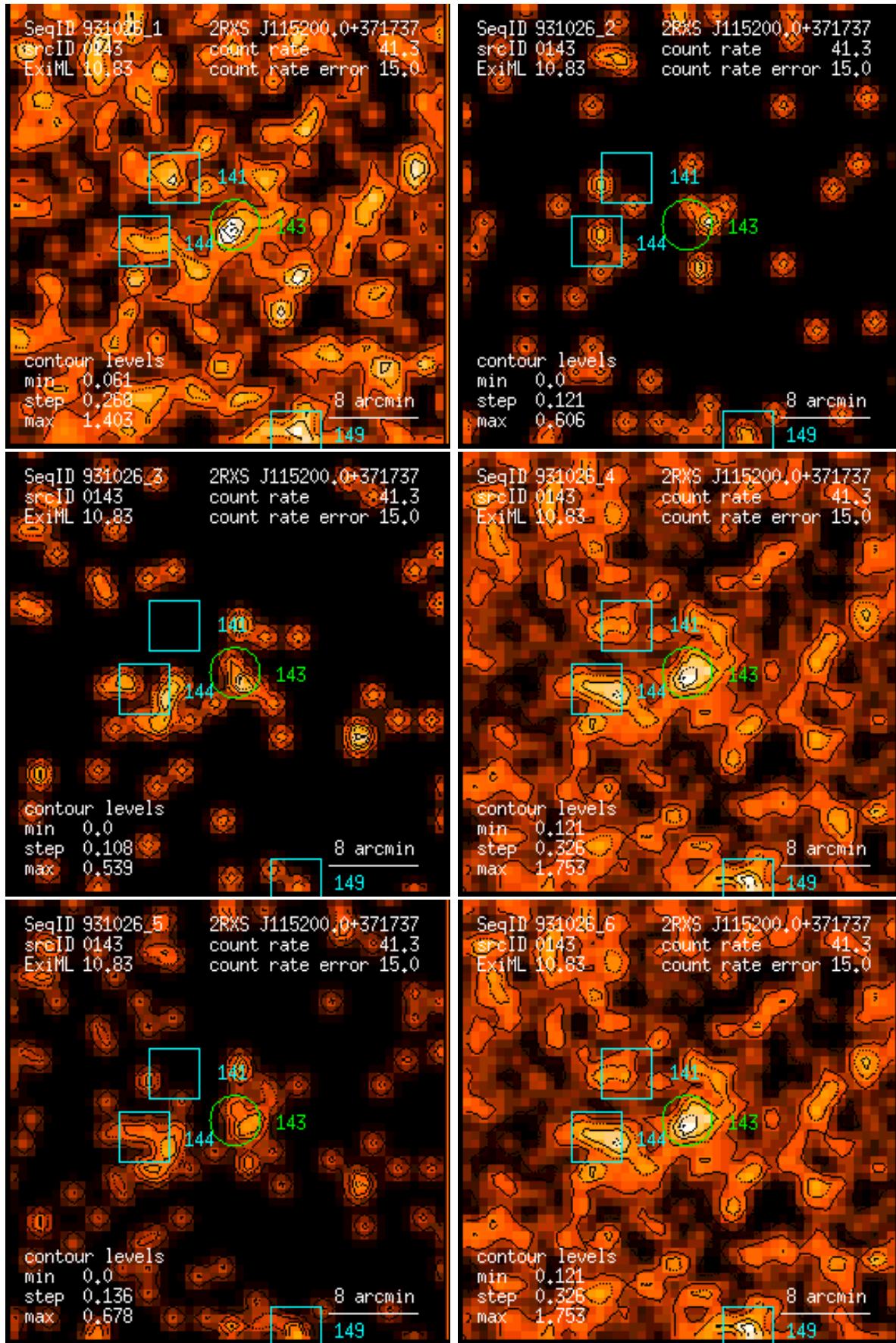
Figure 143: RASS 931026: detection 0143: band rate images, Gaussian filter: (1) PSPC channels 11 – 41, (2) 52 – 90, (3) 91 – 201, (4) 11 – 235, (5) 52 – 201, (6) 11 – 201. Broad band rates in counts/ks. Band rate contour levels in counts/ks/arcmin 2 .
