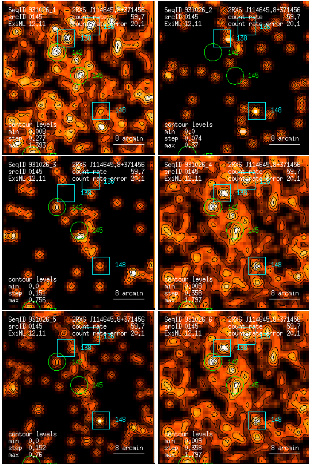
Figure 145: RASS 931026: detection 0145: band rate images, Gaussian filter: (1) PSPC channels 11 – 41, (2) 52 – 90, (3) 91 – 201, (4) 11 – 235, (5) 52 – 201, (6) 11 – 201. Broad band rates in counts/ks. Band rate contour levels in counts/ks/arcmin 2 .
