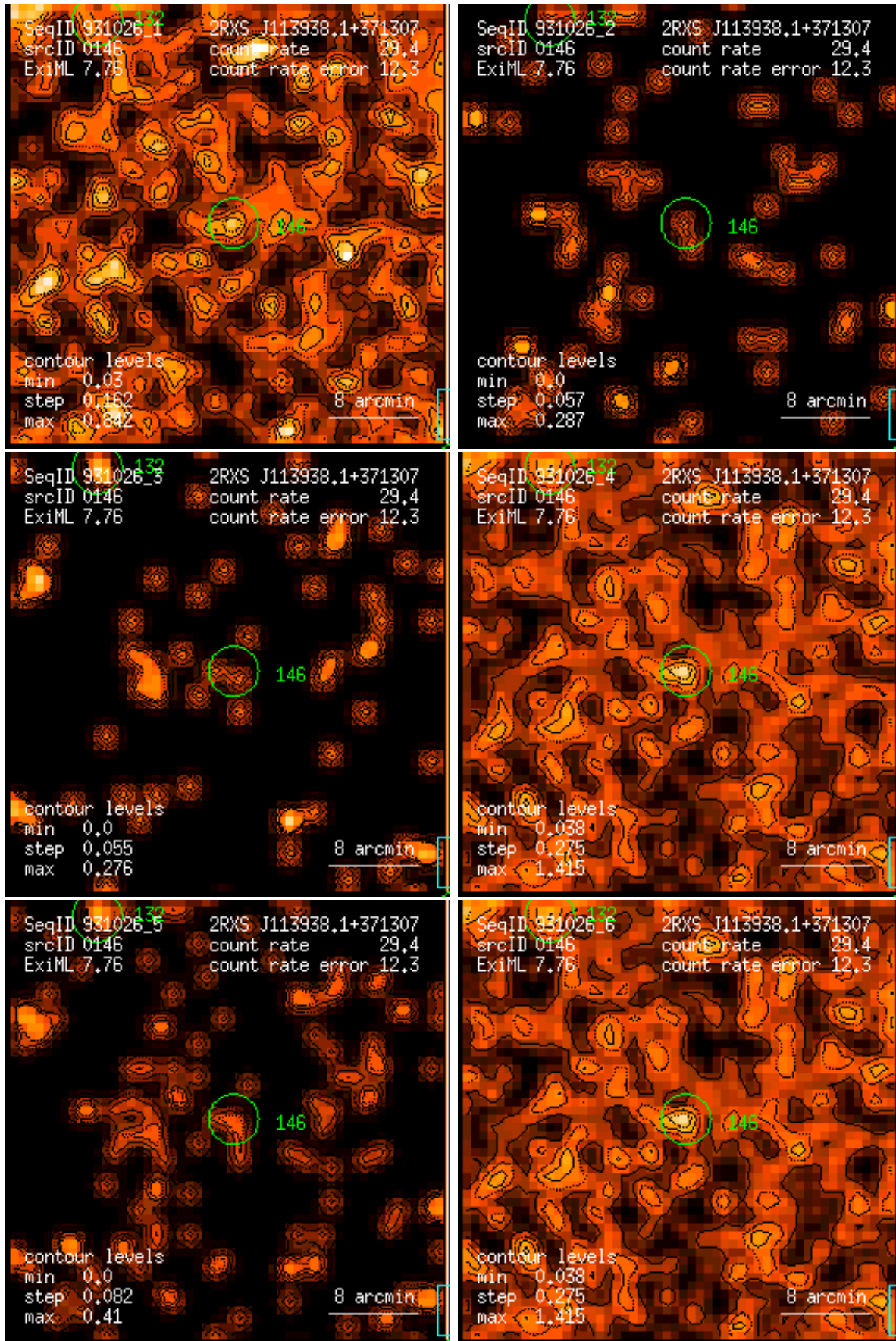
Figure 146: RASS 931026: detection 0146: band rate images, Gaussian filter: (1) PSPC channels 11 – 41, (2) 52 – 90, (3) 91 – 201, (4) 11 – 235, (5) 52 – 201, (6) 11 – 201. Broad band rates in counts/ks. Band rate contour levels in counts/ks/arcmin 2 .
