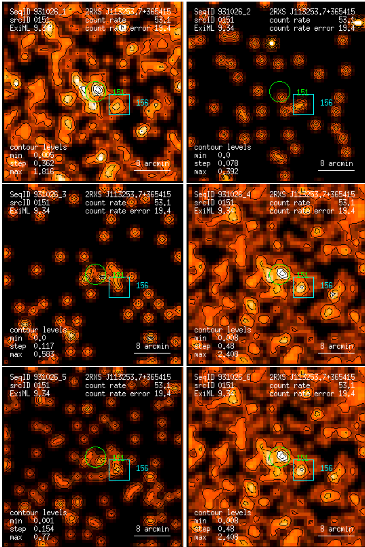
Figure 151: RASS 931026: detection 0151: band rate images, Gaussian filter: (1) PSPC channels 11 – 41, (2) 52 – 90, (3) 91 – 201, (4) 11 – 235, (5) 52 – 201, (6) 11 – 201. Broad band rates in counts/ks. Band rate contour levels in counts/ks/arcmin 2 .
