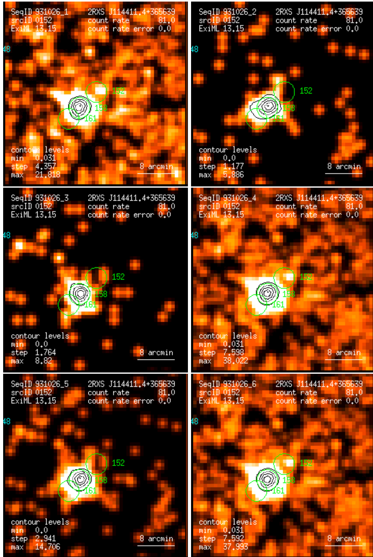
Figure 152: RASS 931026: detection 0152: band rate images, Gaussian filter: (1) PSPC channels 11 – 41, (2) 52 – 90, (3) 91 – 201, (4) 11 – 235, (5) 52 – 201, (6) 11 – 201. Broad band rates in counts/ks. Band rate contour levels in counts/ks/arcmin 2 .
