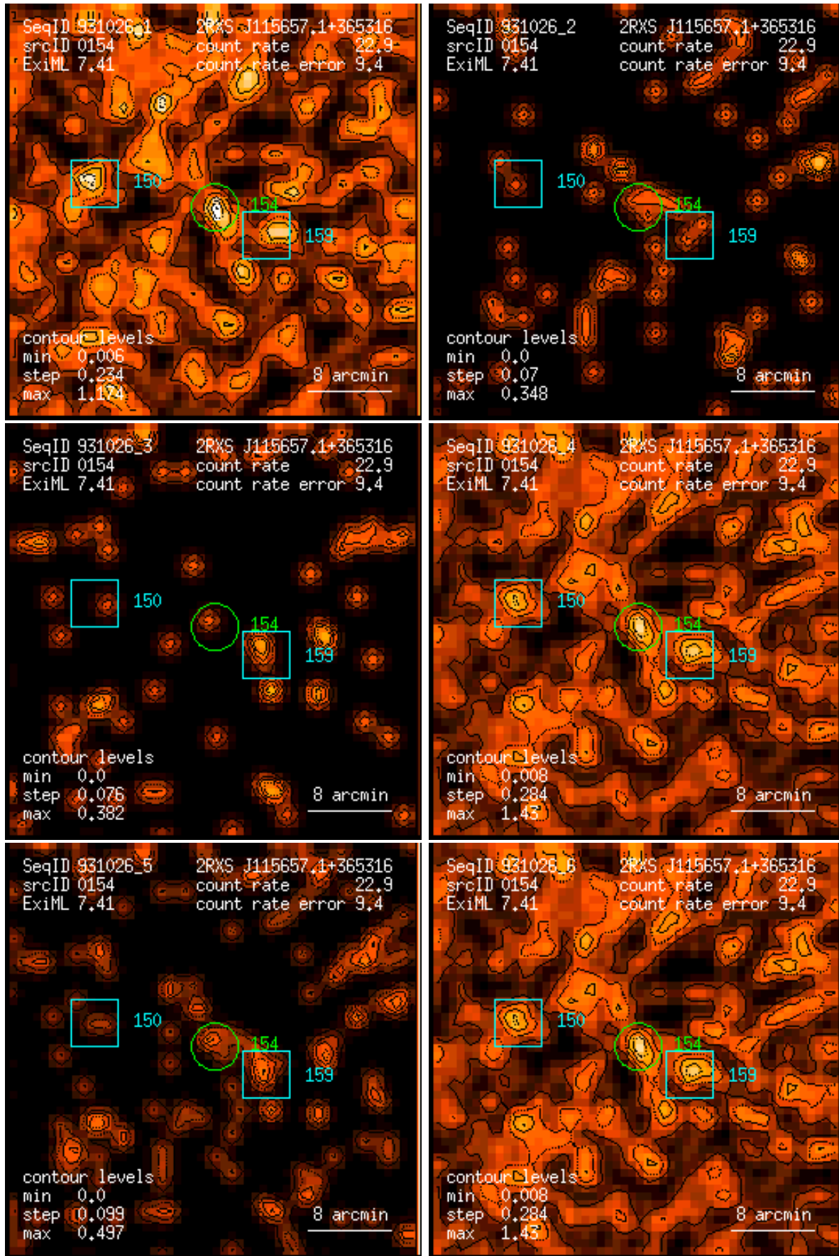
Figure 154: RASS 931026: detection 0154: band rate images, Gaussian filter: (1) PSPC channels 11 – 41, (2) 52 – 90, (3) 91 – 201, (4) 11 – 235, (5) 52 – 201, (6) 11 – 201. Broad band rates in counts/ks. Band rate contour levels in counts/ks/arcmin 2 .
