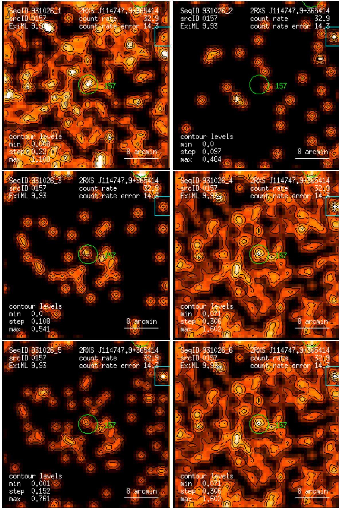
Figure 157: RASS 931026: detection 0157: band rate images, Gaussian filter: (1) PSPC channels 11 – 41, (2) 52 – 90, (3) 91 – 201, (4) 11 – 235, (5) 52 – 201, (6) 11 – 201. Broad band rates in counts/ks. Band rate contour levels in counts/ks/arcmin 2 .
