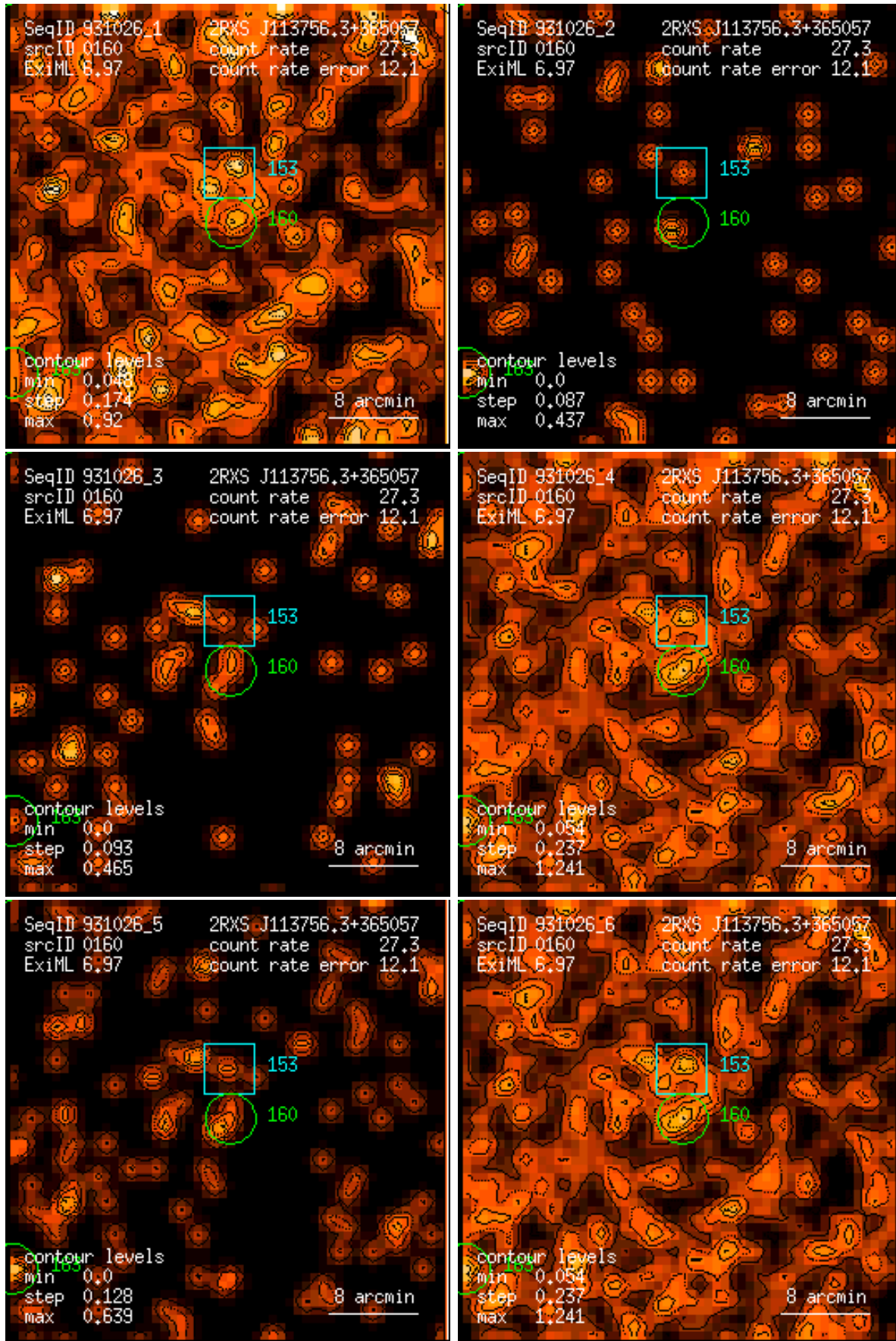
Figure 160: RASS 931026: detection 0160: band rate images, Gaussian filter: (1) PSPC channels 11 – 41, (2) 52 – 90, (3) 91 – 201, (4) 11 – 235, (5) 52 – 201, (6) 11 – 201. Broad band rates in counts/ks. Band rate contour levels in counts/ks/arcmin 2 .
