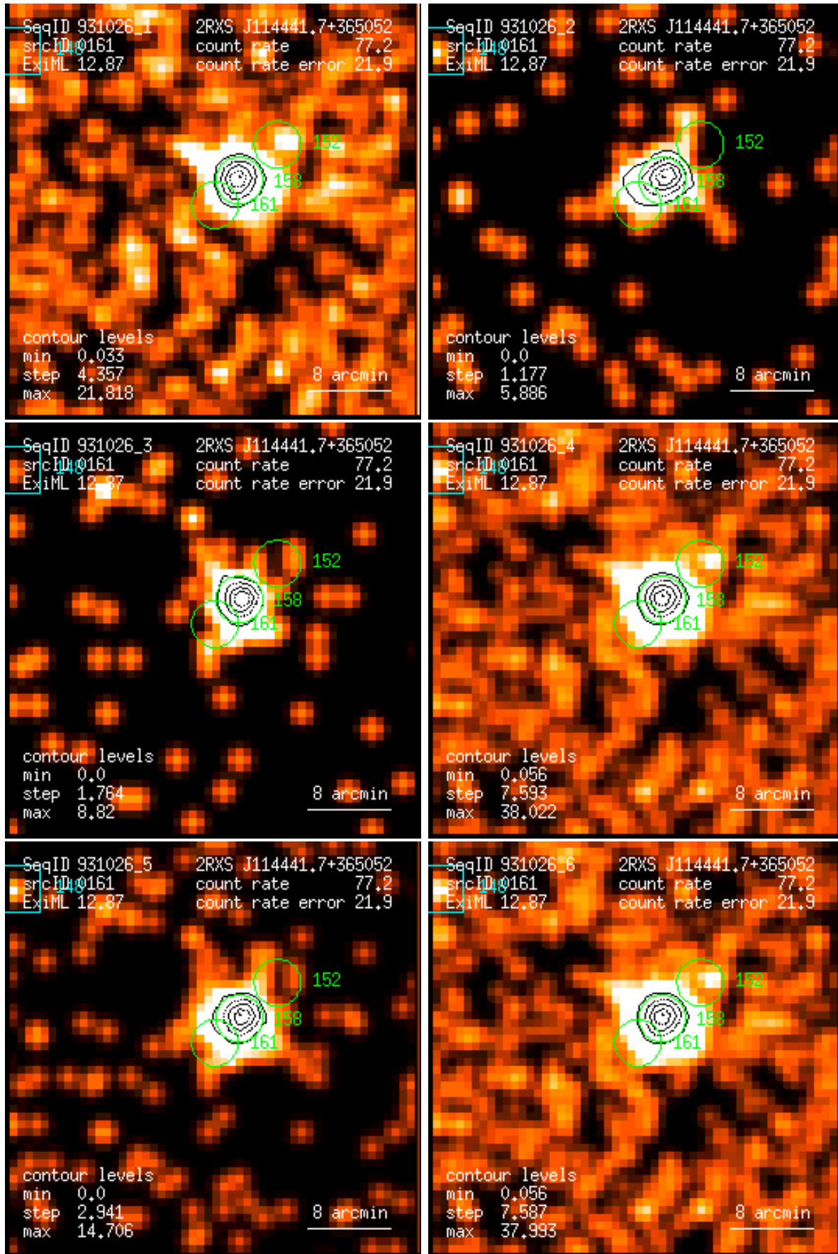
Figure 161: RASS 931026: detection 0161: band rate images, Gaussian filter: (1) PSPC channels 11 – 41, (2) 52 – 90, (3) 91 – 201, (4) 11 – 235, (5) 52 – 201, (6) 11 – 201. Broad band rates in counts/ks. Band rate contour levels in counts/ks/arcmin 2 .
