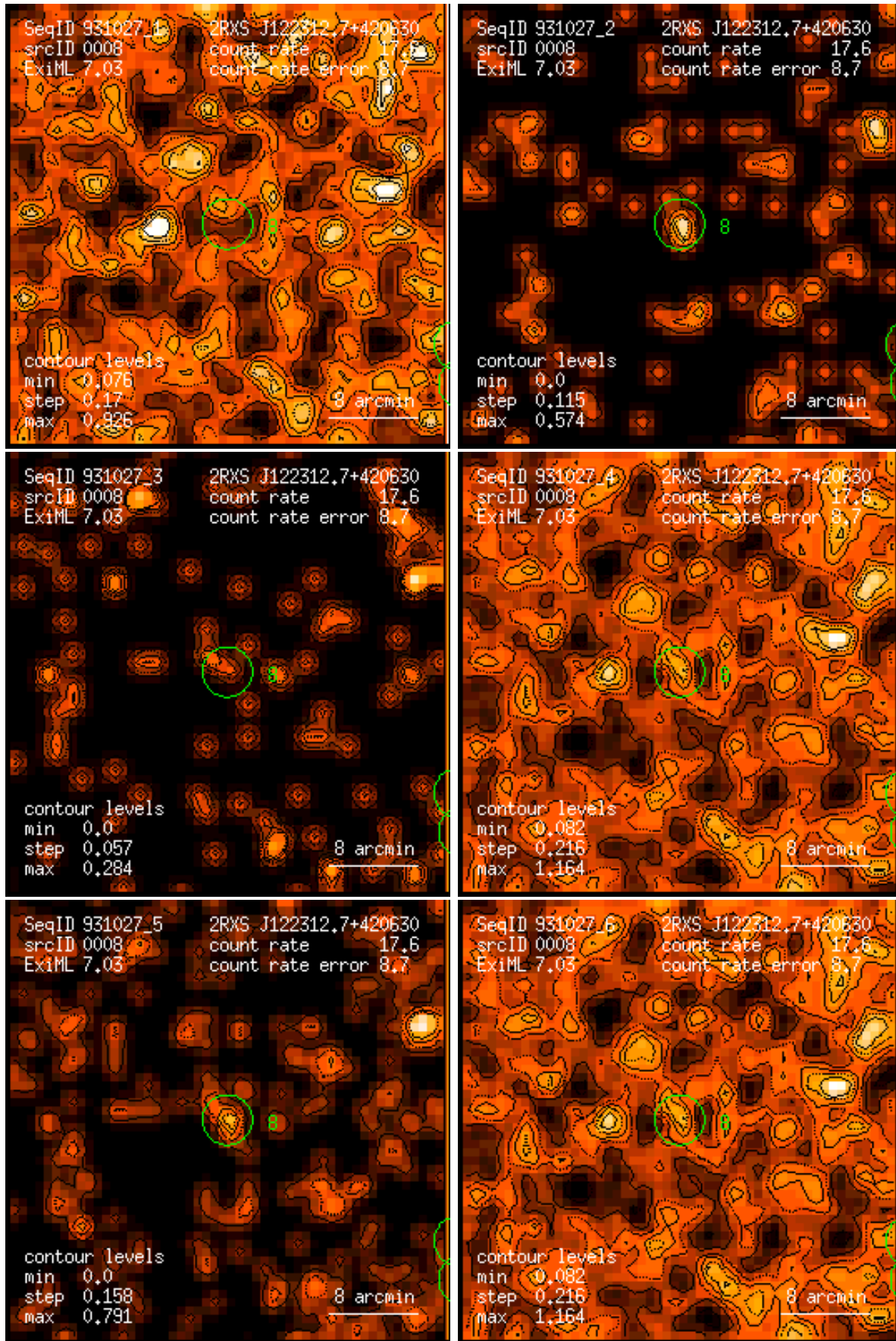
Figure 8: RASS 931027: detection 0008: band rate images, Gaussian filter: (1) PSPC channels 11 – 41, (2) 52 – 90, (3) 91 – 201, (4) 11 – 235, (5) 52 – 201, (6) 11 – 201. Broad band rates in counts/ks. Band rate contour levels in counts/ks/arcmin 2 .
