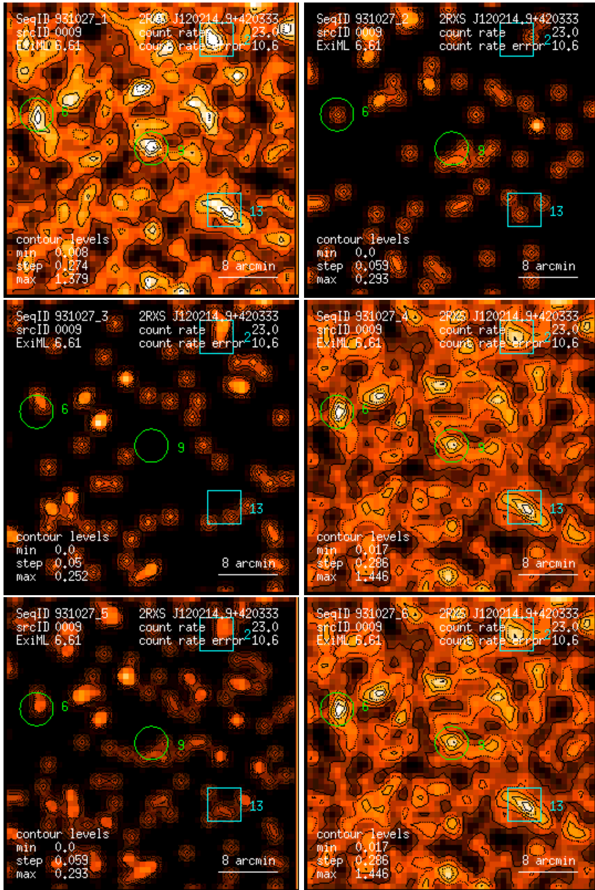
Figure 9: RASS 931027: detection 0009: band rate images, Gaussian filter: (1) PSPC channels 11 – 41, (2) 52 – 90, (3) 91 – 201, (4) 11 – 235, (5) 52 – 201, (6) 11 – 201. Broad band rates in counts/ks. Band rate contour levels in counts/ks/arcmin 2 .
