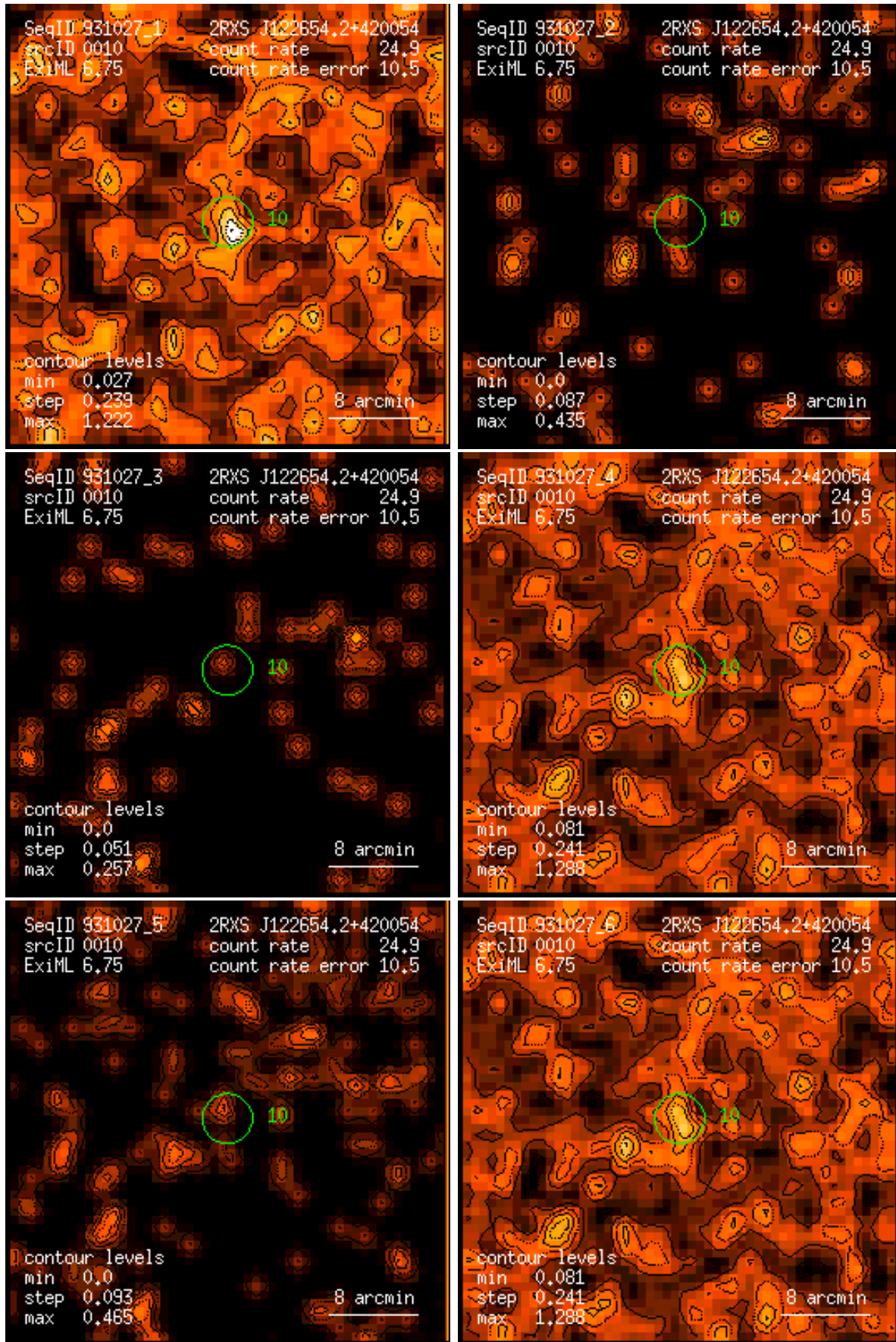
Figure 10: RASS 931027: detection 0010: band rate images, Gaussian filter: (1) PSPC channels 11 – 41, (2) 52 – 90, (3) 91 – 201, (4) 11 – 235, (5) 52 – 201, (6) 11 – 201. Broad band rates in counts/ks. Band rate contour levels in counts/ks/arcmin 2 .
