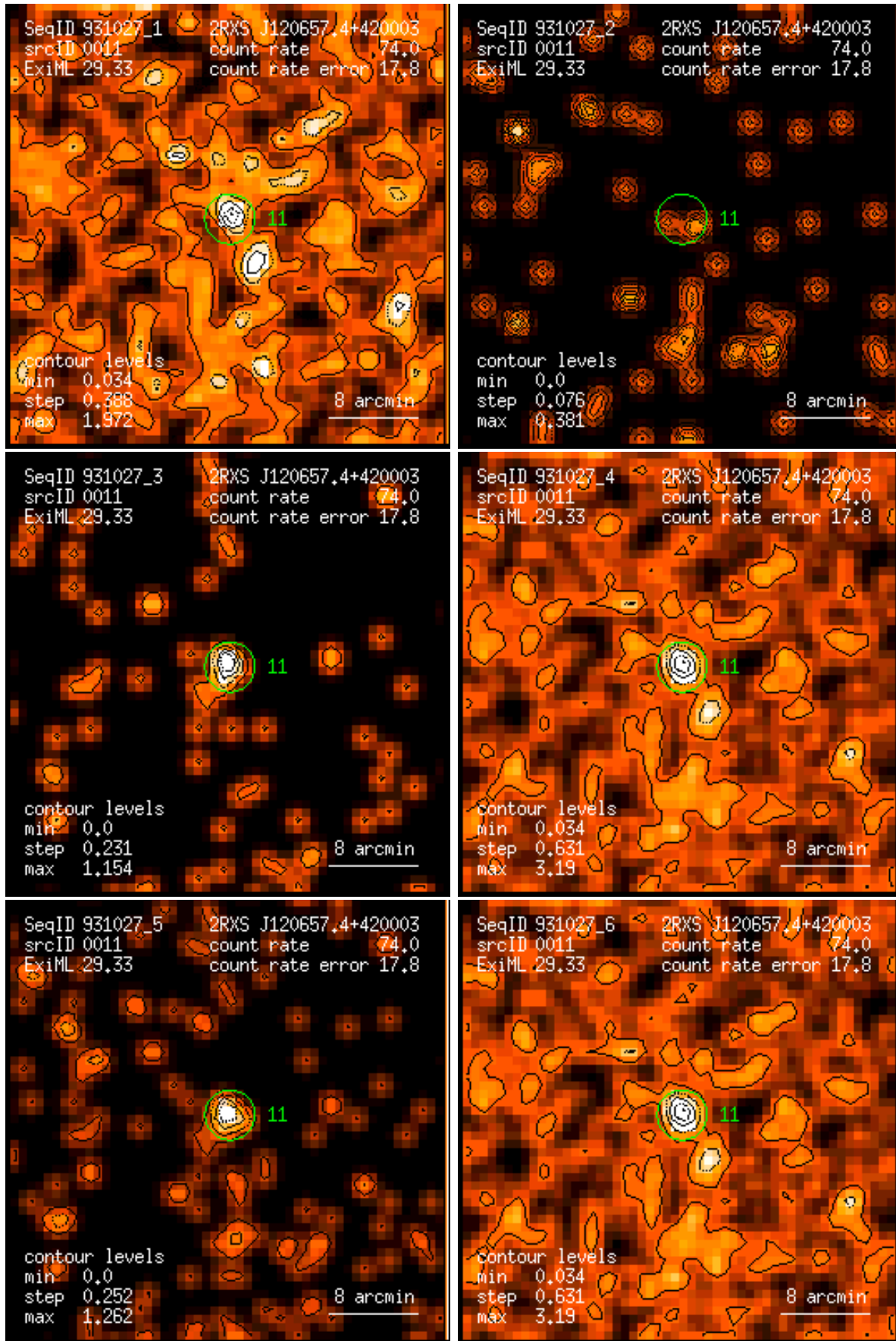
Figure 11: RASS 931027: detection 0011: band rate images, Gaussian filter: (1) PSPC channels 11 – 41, (2) 52 – 90, (3) 91 – 201, (4) 11 – 235, (5) 52 – 201, (6) 11 – 201. Broad band rates in counts/ks. Band rate contour levels in counts/ks/arcmin 2 .
