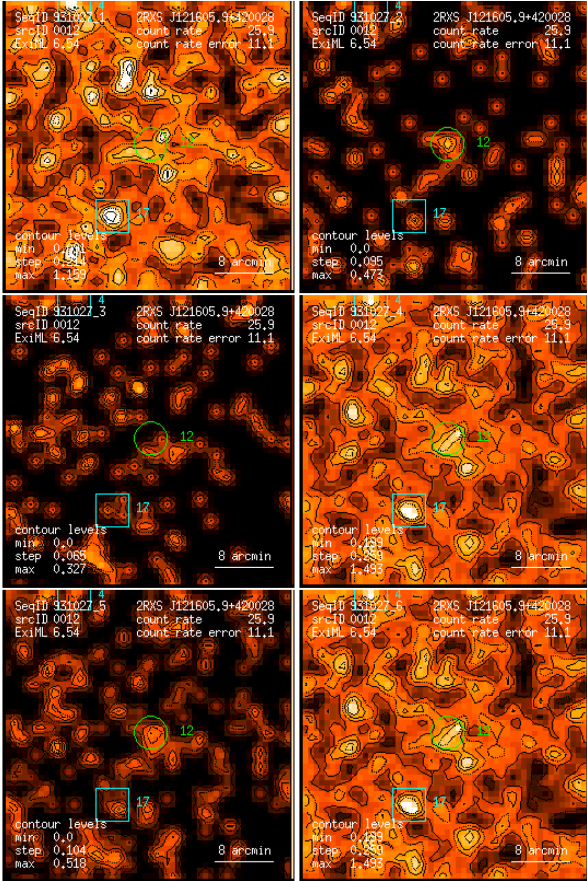
Figure 12: RASS 931027: detection 0012: band rate images, Gaussian filter: (1) PSPC channels 11 – 41, (2) 52 – 90, (3) 91 – 201, (4) 11 – 235, (5) 52 – 201, (6) 11 – 201. Broad band rates in counts/ks. Band rate contour levels in counts/ks/arcmin 2 .
