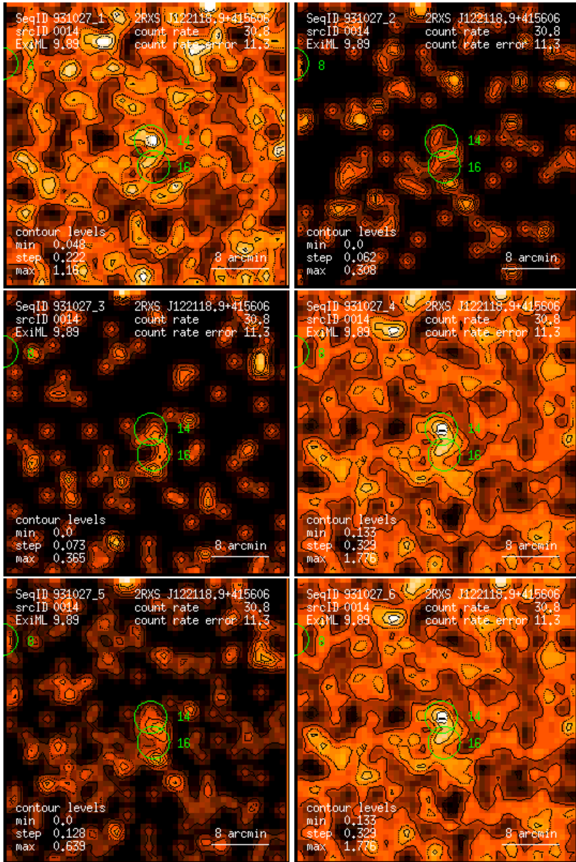
Figure 14: RASS 931027: detection 0014: band rate images, Gaussian filter: (1) PSPC channels 11 – 41, (2) 52 – 90, (3) 91 – 201, (4) 11 – 235, (5) 52 – 201, (6) 11 – 201. Broad band rates in counts/ks. Band rate contour levels in counts/ks/arcmin 2 .
