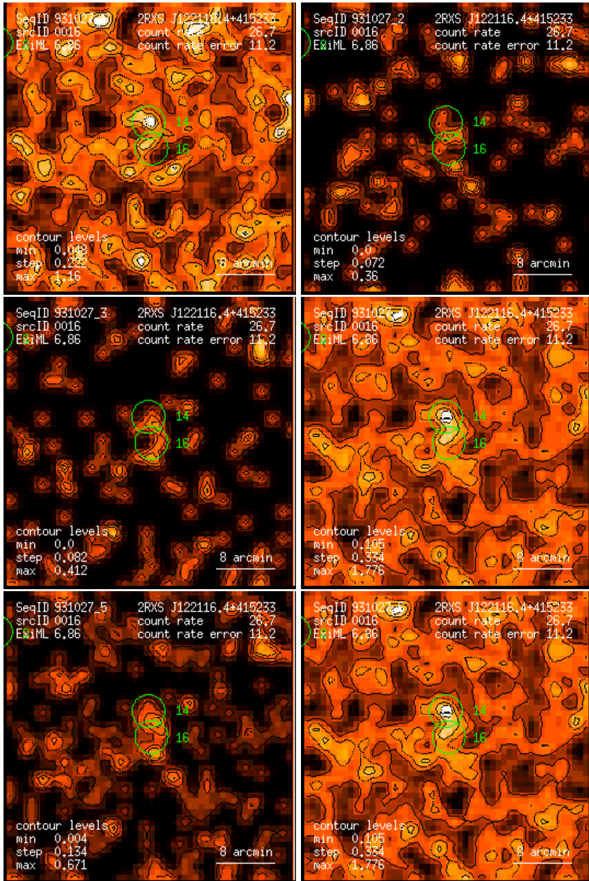
Figure 16: RASS 931027: detection 0016: band rate images, Gaussian filter: (1) PSPC channels 11 – 41, (2) 52 – 90, (3) 91 – 201, (4) 11 – 235, (5) 52 – 201, (6) 11 – 201. Broad band rates in counts/ks. Band rate contour levels in counts/ks/arcmin 2 .
