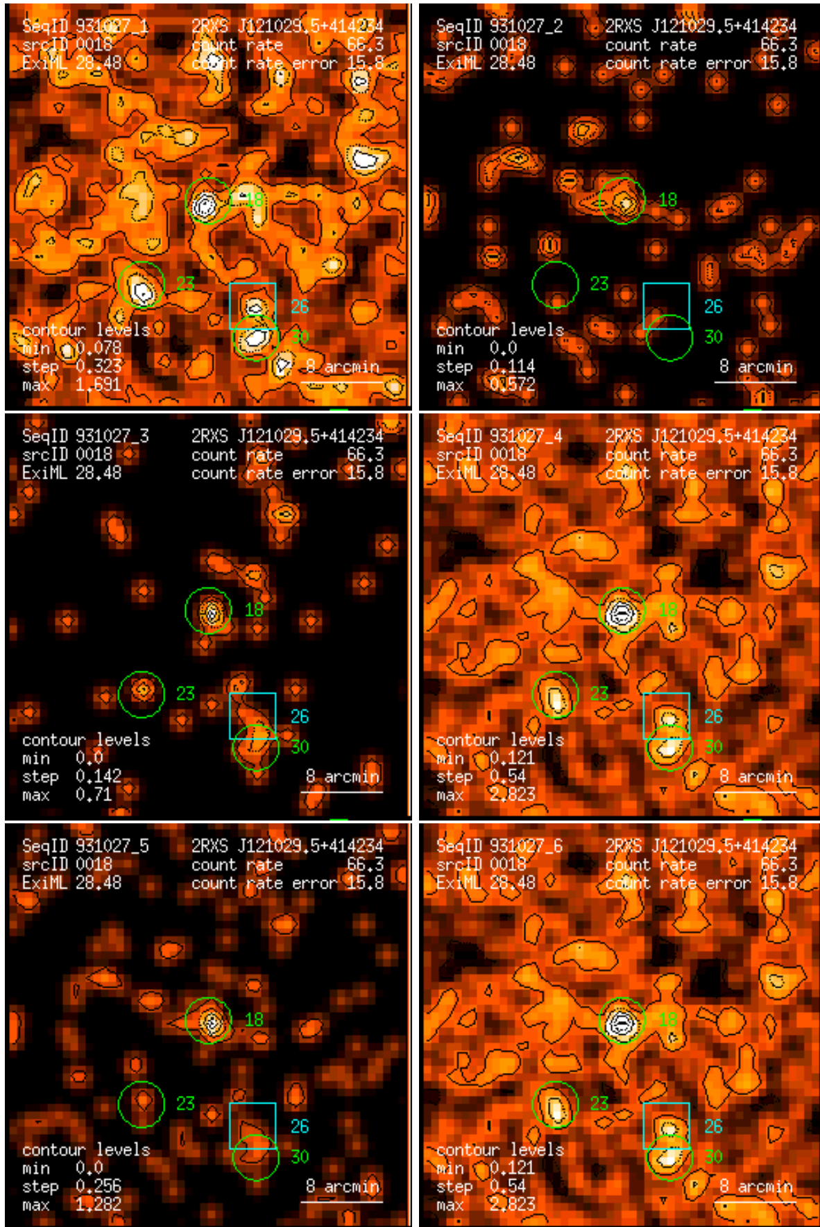
Figure 18: RASS 931027: detection 0018: band rate images, Gaussian filter: (1) PSPC channels 11 – 41, (2) 52 – 90, (3) 91 – 201, (4) 11 – 235, (5) 52 – 201, (6) 11 – 201. Broad band rates in counts/ks. Band rate contour levels in counts/ks/arcmin 2 .
