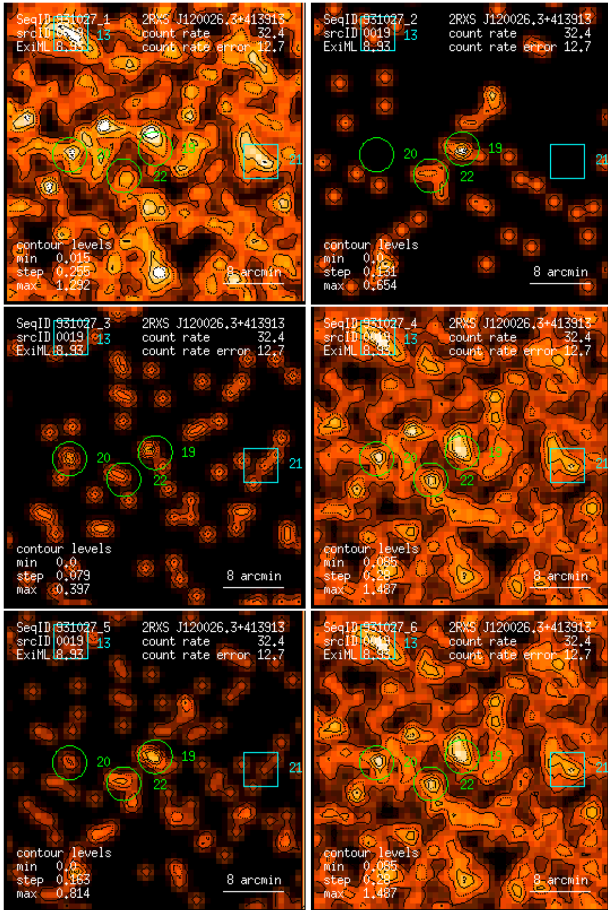
Figure 19: RASS 931027: detection 0019: band rate images, Gaussian filter: (1) PSPC channels 11 – 41, (2) 52 – 90, (3) 91 – 201, (4) 11 – 235, (5) 52 – 201, (6) 11 – 201. Broad band rates in counts/ks. Band rate contour levels in counts/ks/arcmin 2 .
