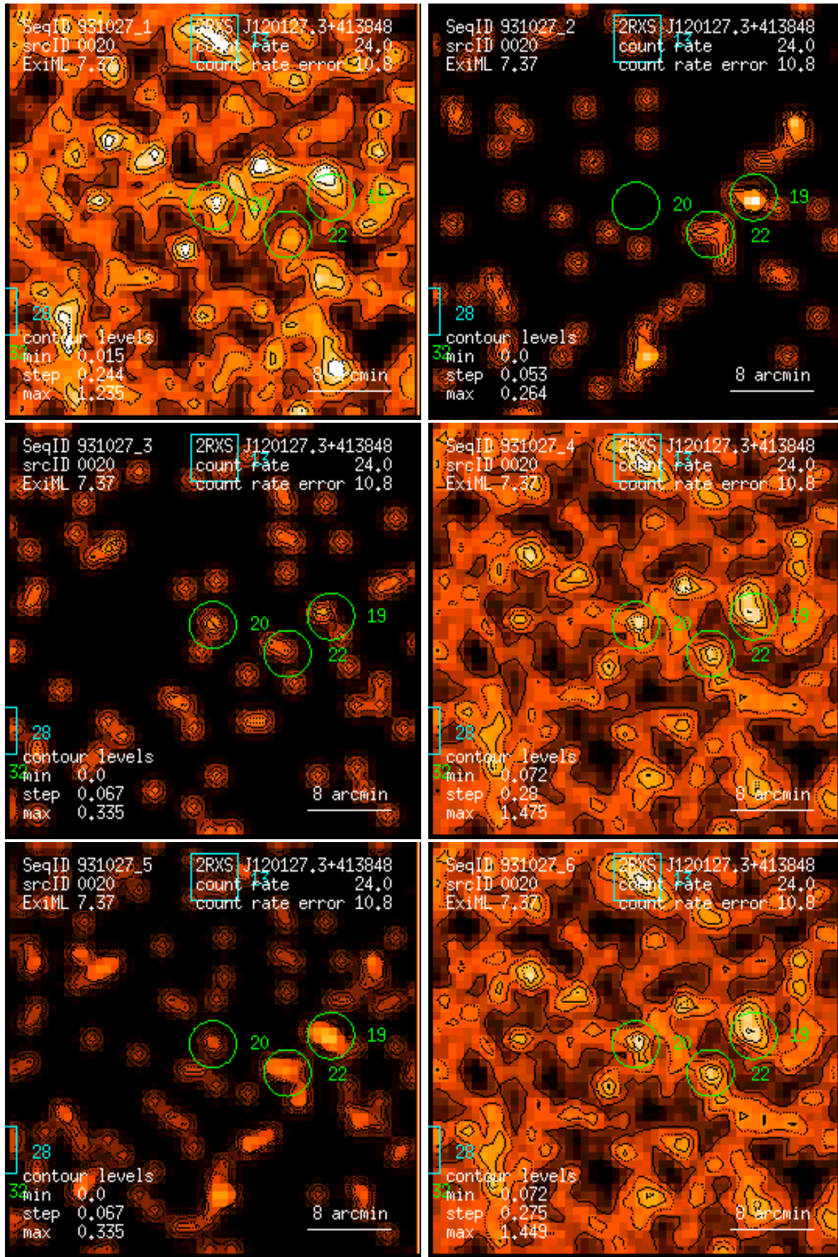
Figure 20: RASS 931027: detection 0020: band rate images, Gaussian filter: (1) PSPC channels 11 – 41, (2) 52 – 90, (3) 91 – 201, (4) 11 – 235, (5) 52 – 201, (6) 11 – 201. Broad band rates in counts/ks. Band rate contour levels in counts/ks/arcmin 2 .
