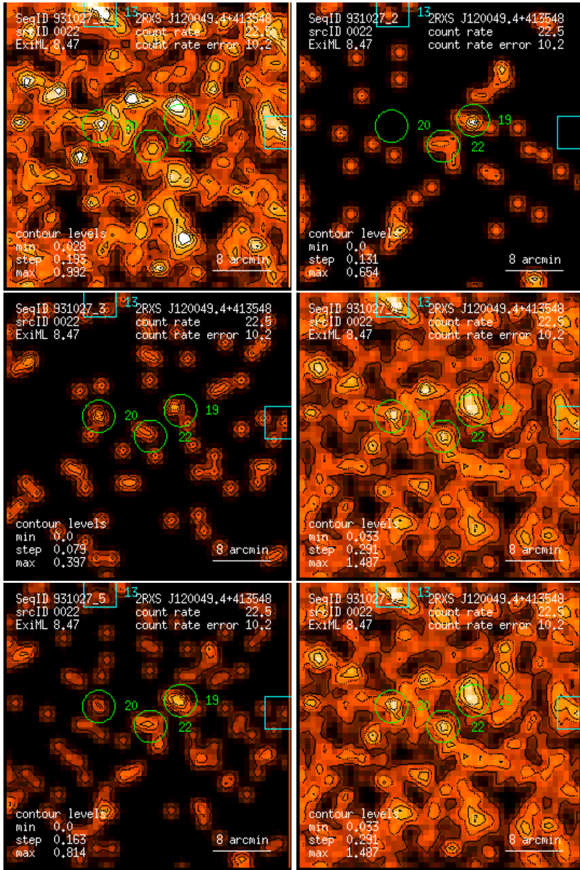
Figure 22: RASS 931027: detection 0022: band rate images, Gaussian filter: (1) PSPC channels 11 – 41, (2) 52 – 90, (3) 91 – 201, (4) 11 – 235, (5) 52 – 201, (6) 11 – 201. Broad band rates in counts/ks. Band rate contour levels in counts/ks/arcmin 2 .
