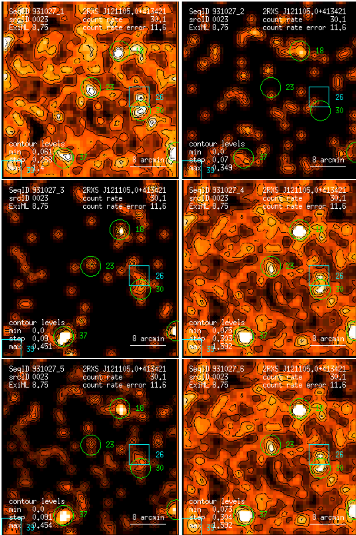
Figure 23: RASS 931027: detection 0023: band rate images, Gaussian filter: (1) PSPC channels 11 – 41, (2) 52 – 90, (3) 91 – 201, (4) 11 – 235, (5) 52 – 201, (6) 11 – 201. Broad band rates in counts/ks. Band rate contour levels in counts/ks/arcmin 2 .
