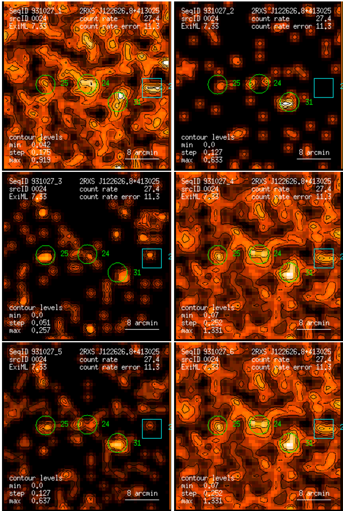
Figure 24: RASS 931027: detection 0024: band rate images, Gaussian filter: (1) PSPC channels 11 – 41, (2) 52 – 90, (3) 91 – 201, (4) 11 – 235, (5) 52 – 201, (6) 11 – 201. Broad band rates in counts/ks. Band rate contour levels in counts/ks/arcmin 2 .
