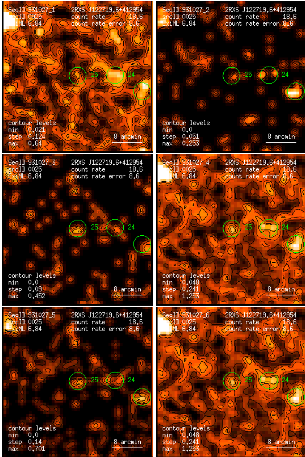
Figure 25: RASS 931027: detection 0025: band rate images, Gaussian filter: (1) PSPC channels 11 – 41, (2) 52 – 90, (3) 91 – 201, (4) 11 – 235, (5) 52 – 201, (6) 11 – 201. Broad band rates in counts/ks. Band rate contour levels in counts/ks/arcmin 2 .
