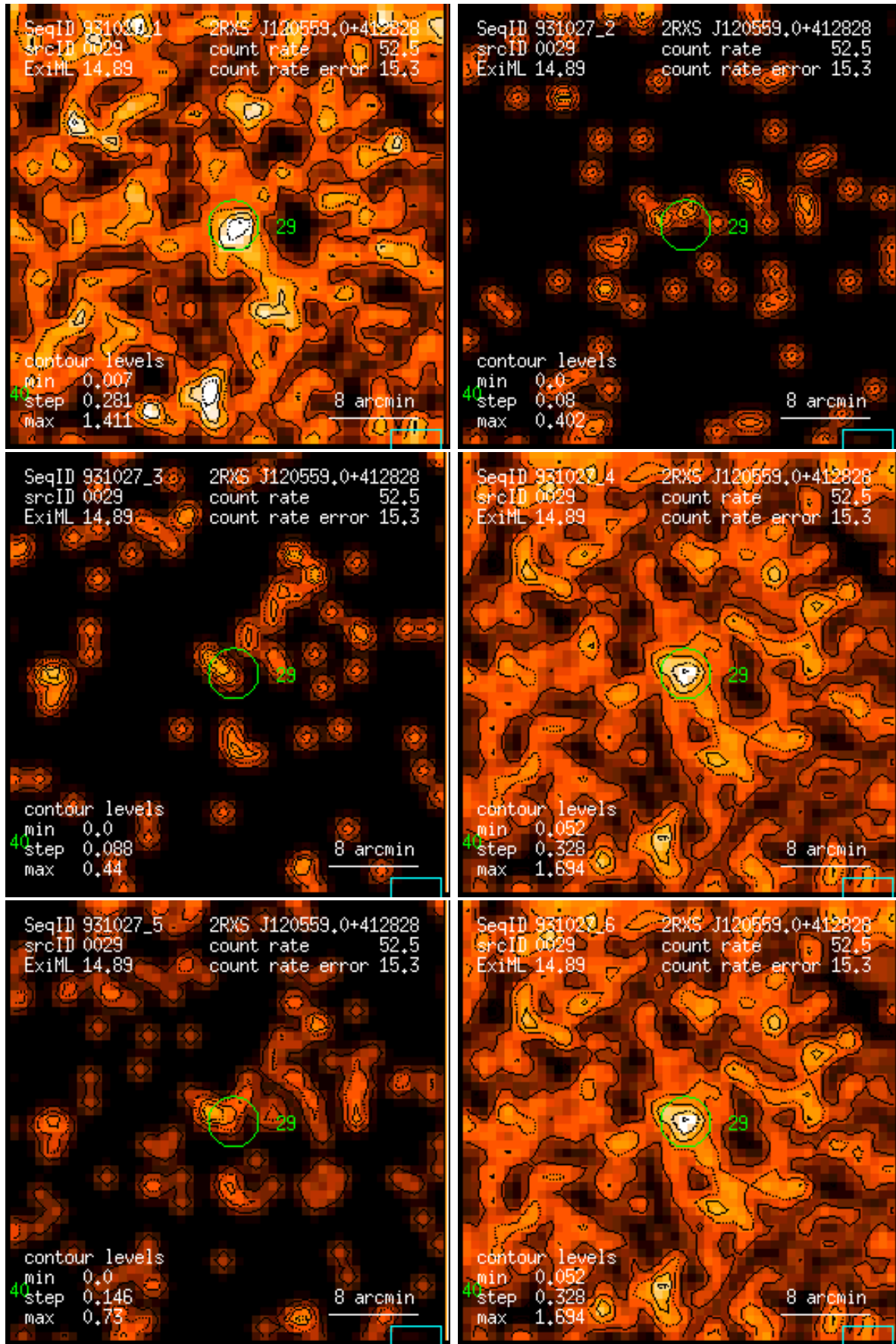
Figure 29: RASS 931027: detection 0029: band rate images, Gaussian filter: (1) PSPC channels 11 – 41, (2) 52 – 90, (3) 91 – 201, (4) 11 – 235, (5) 52 – 201, (6) 11 – 201. Broad band rates in counts/ks. Band rate contour levels in counts/ks/arcmin 2 .
