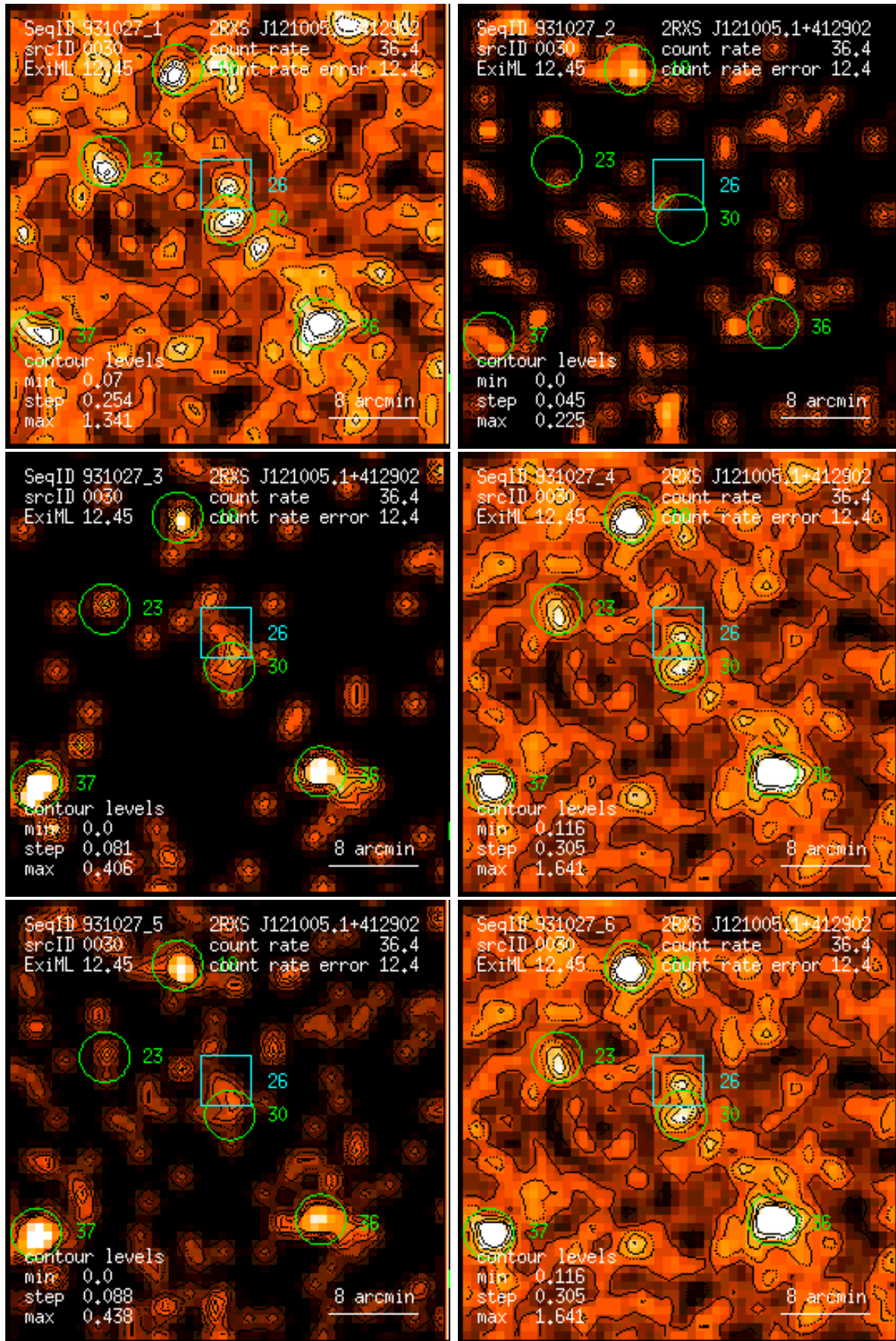
Figure 30: RASS 931027: detection 0030: band rate images, Gaussian filter: (1) PSPC channels 11 – 41, (2) 52 – 90, (3) 91 – 201, (4) 11 – 235, (5) 52 – 201, (6) 11 – 201. Broad band rates in counts/ks. Band rate contour levels in counts/ks/arcmin 2 .
