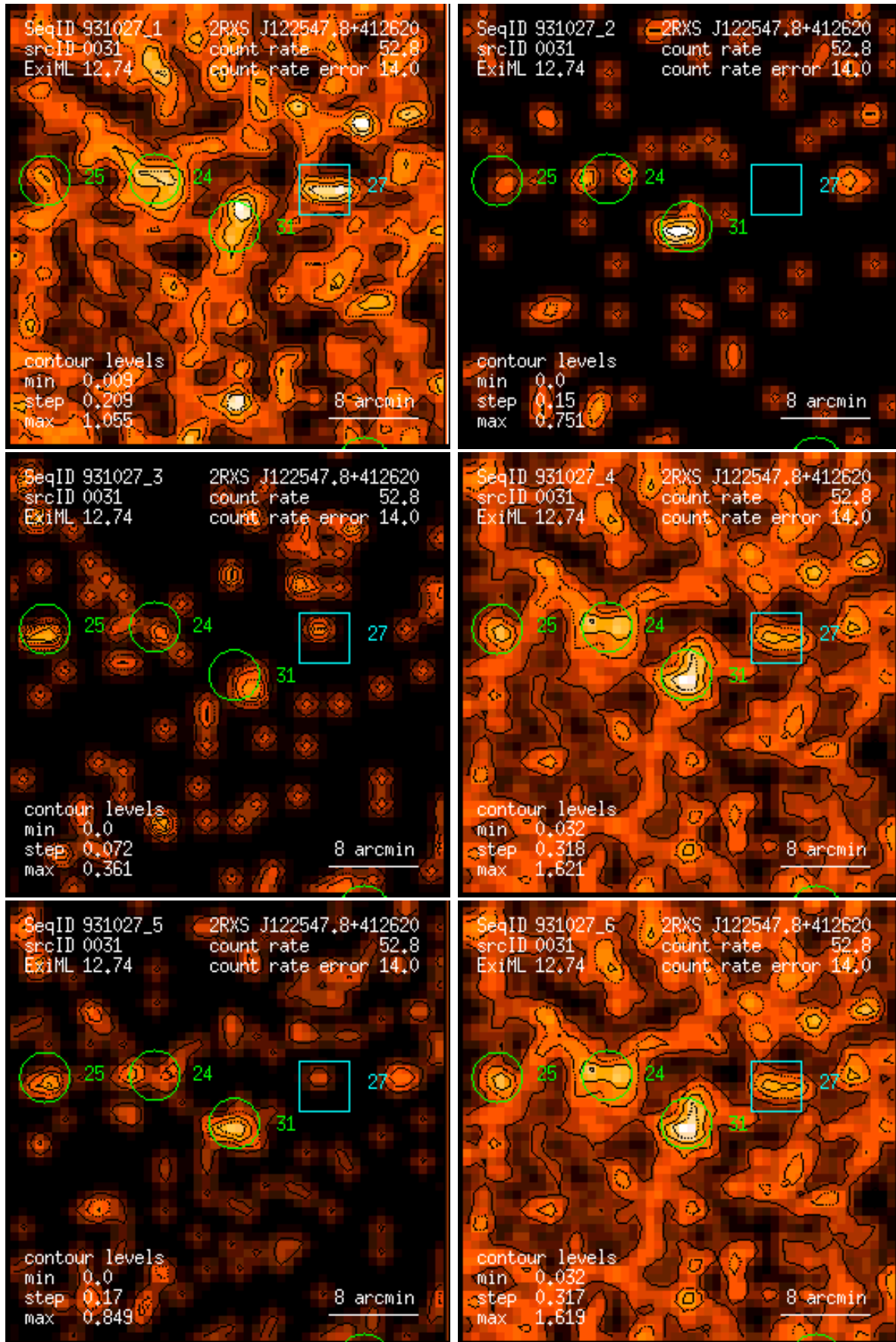
Figure 31: RASS 931027: detection 0031: band rate images, Gaussian filter: (1) PSPC channels 11 – 41, (2) 52 – 90, (3) 91 – 201, (4) 11 – 235, (5) 52 – 201, (6) 11 – 201. Broad band rates in counts/ks. Band rate contour levels in counts/ks/arcmin 2 .
