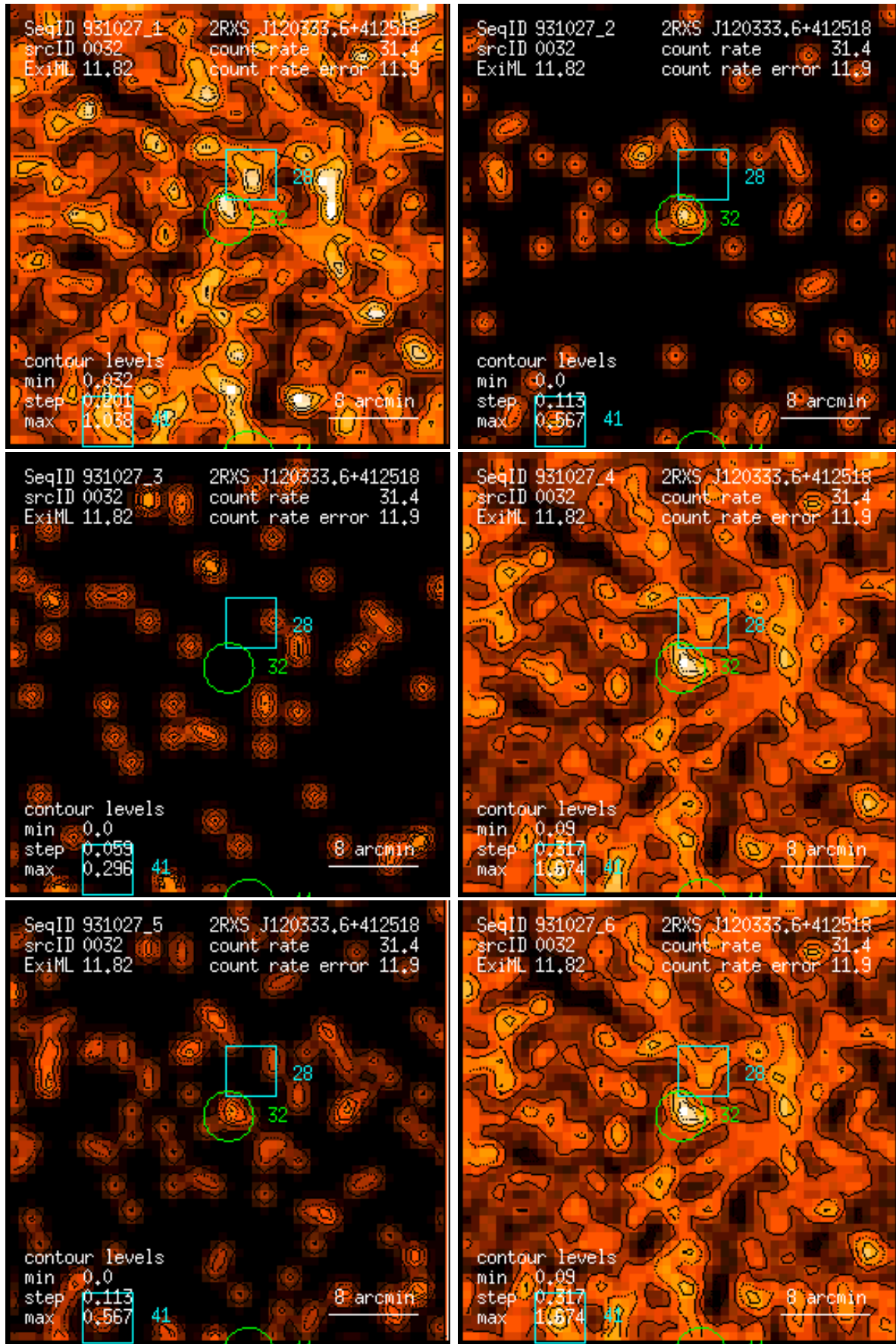
Figure 32: RASS 931027: detection 0032: band rate images, Gaussian filter: (1) PSPC channels 11 – 41, (2) 52 – 90, (3) 91 – 201, (4) 11 – 235, (5) 52 – 201, (6) 11 – 201. Broad band rates in counts/ks. Band rate contour levels in counts/ks/arcmin 2 .
