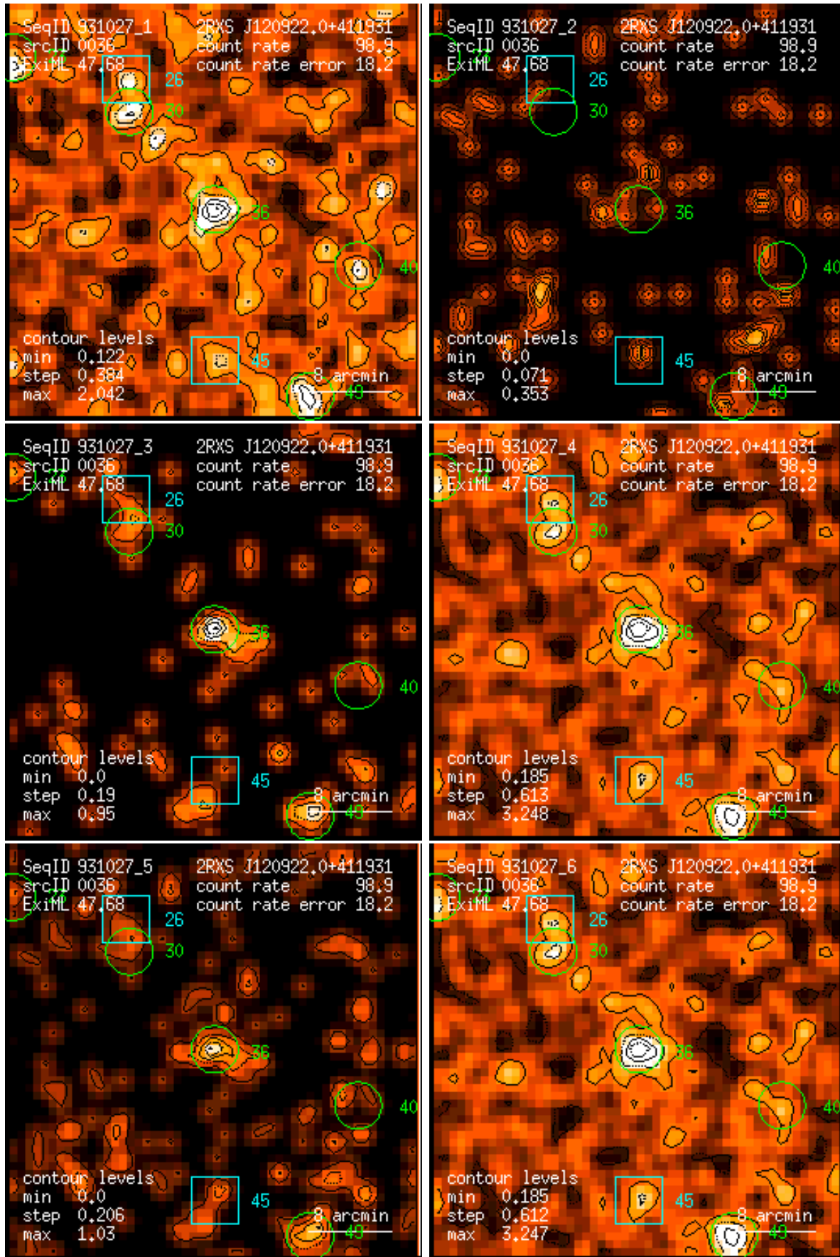
Figure 36: RASS 931027: detection 0036: band rate images, Gaussian filter: (1) PSPC channels 11 – 41, (2) 52 – 90, (3) 91 – 201, (4) 11 – 235, (5) 52 – 201, (6) 11 – 201. Broad band rates in counts/ks. Band rate contour levels in counts/ks/arcmin 2 .
