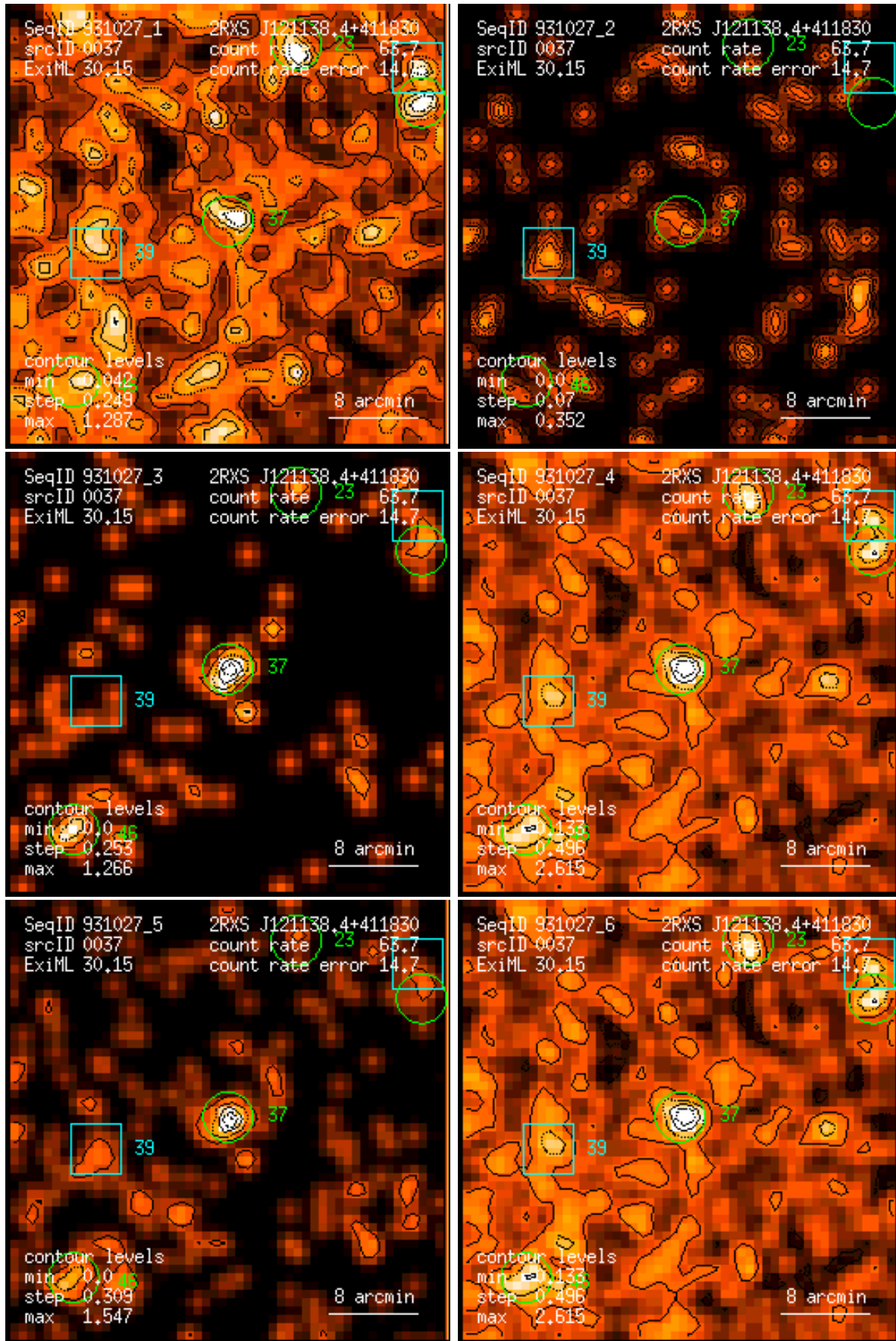
Figure 37: RASS 931027: detection 0037: band rate images, Gaussian filter: (1) PSPC channels 11 – 41, (2) 52 – 90, (3) 91 – 201, (4) 11 – 235, (5) 52 – 201, (6) 11 – 201. Broad band rates in counts/ks. Band rate contour levels in counts/ks/arcmin 2 .
