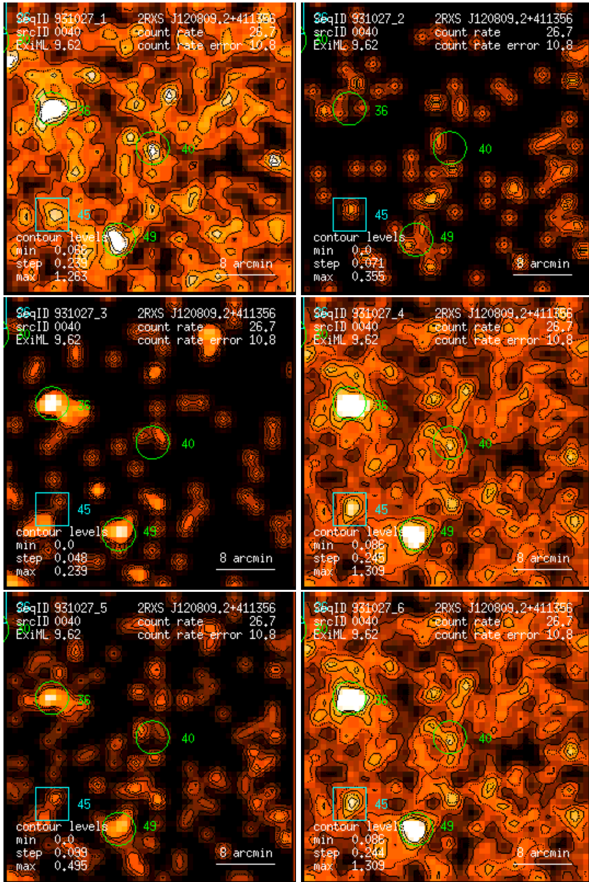
Figure 40: RASS 931027: detection 0040: band rate images, Gaussian filter: (1) PSPC channels 11 – 41, (2) 52 – 90, (3) 91 – 201, (4) 11 – 235, (5) 52 – 201, (6) 11 – 201. Broad band rates in counts/ks. Band rate contour levels in counts/ks/arcmin 2 .
