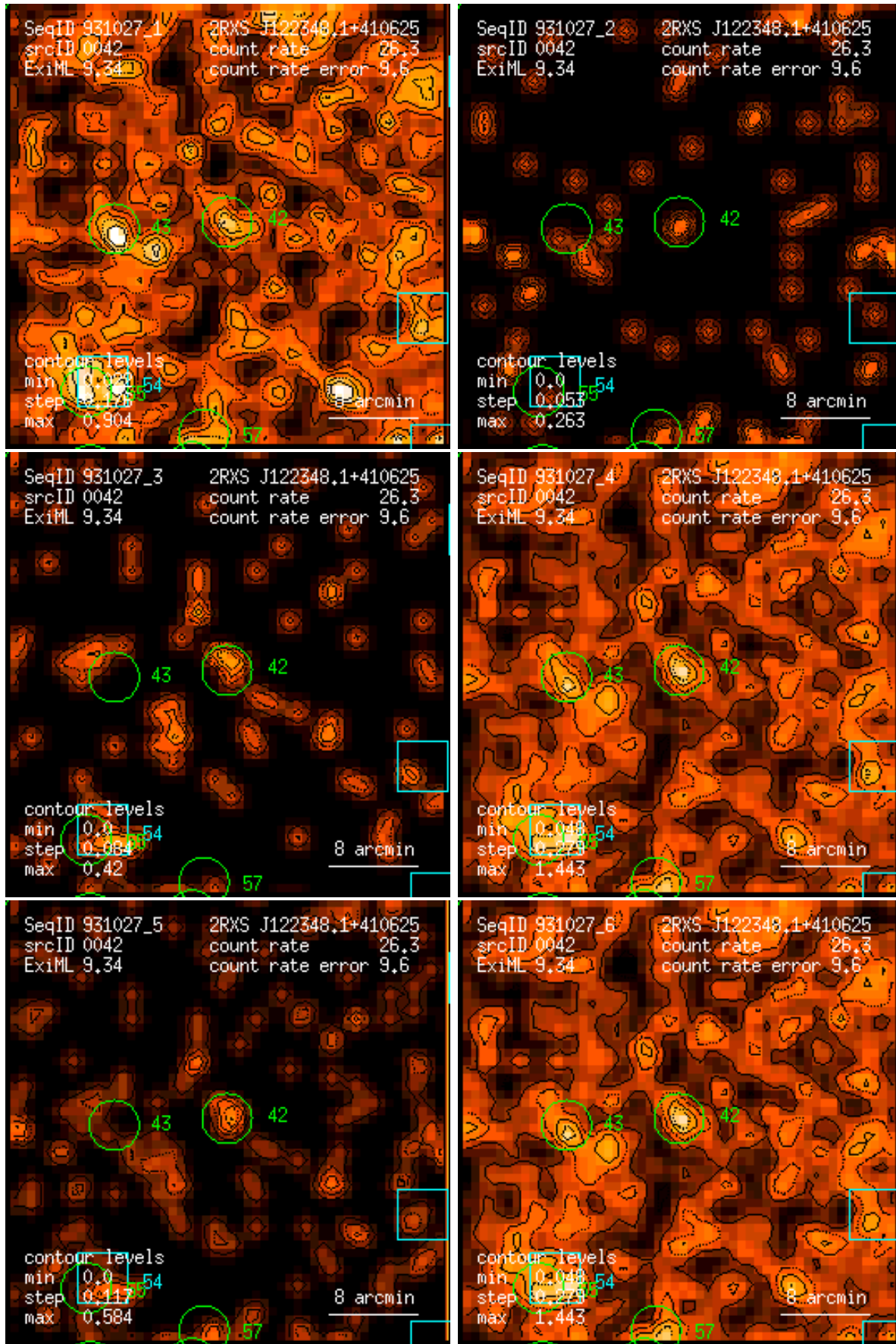
Figure 42: RASS 931027: detection 0042: band rate images, Gaussian filter: (1) PSPC channels 11 – 41, (2) 52 – 90, (3) 91 – 201, (4) 11 – 235, (5) 52 – 201, (6) 11 – 201. Broad band rates in counts/ks. Band rate contour levels in counts/ks/arcmin 2 .
