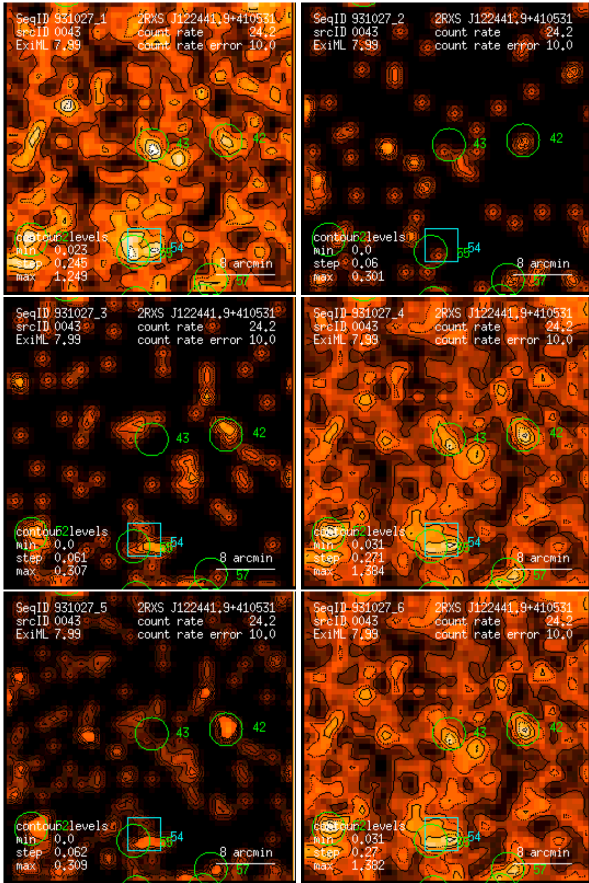
Figure 43: RASS 931027: detection 0043: band rate images, Gaussian filter: (1) PSPC channels 11 – 41, (2) 52 – 90, (3) 91 – 201, (4) 11 – 235, (5) 52 – 201, (6) 11 – 201. Broad band rates in counts/ks. Band rate contour levels in counts/ks/arcmin 2 .
