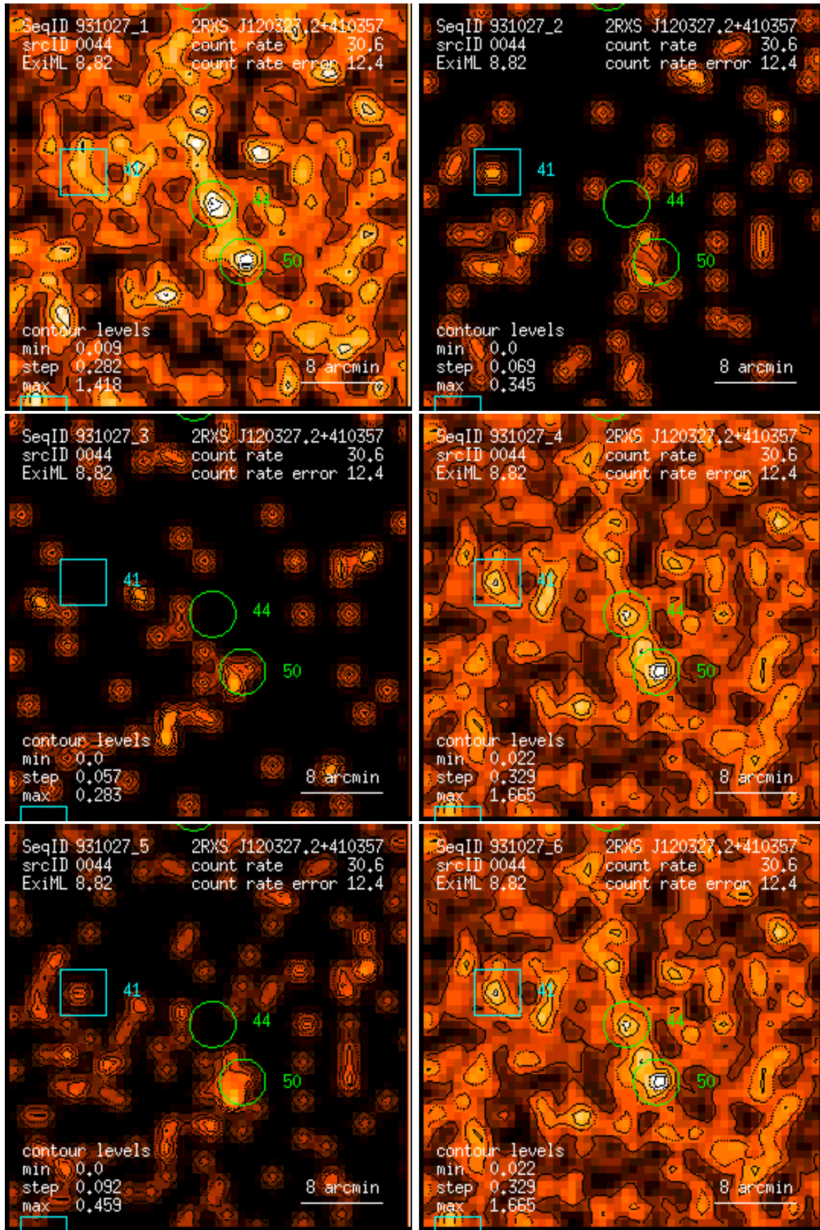
Figure 44: RASS 931027: detection 0044: band rate images, Gaussian filter: (1) PSPC channels 11 – 41, (2) 52 – 90, (3) 91 – 201, (4) 11 – 235, (5) 52 – 201, (6) 11 – 201. Broad band rates in counts/ks. Band rate contour levels in counts/ks/arcmin 2 .
