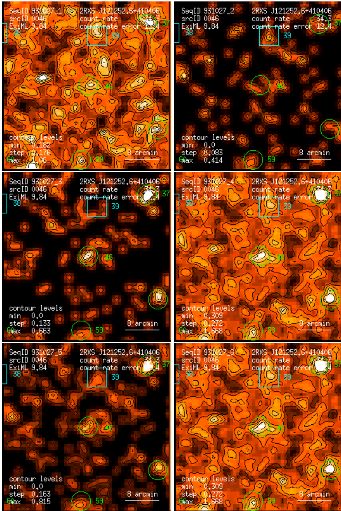
Figure 46: RASS 931027: detection 0046: band rate images, Gaussian filter: (1) PSPC channels 11 – 41, (2) 52 – 90, (3) 91 – 201, (4) 11 – 235, (5) 52 – 201, (6) 11 – 201. Broad band rates in counts/ks. Band rate contour levels in counts/ks/arcmin 2 .
