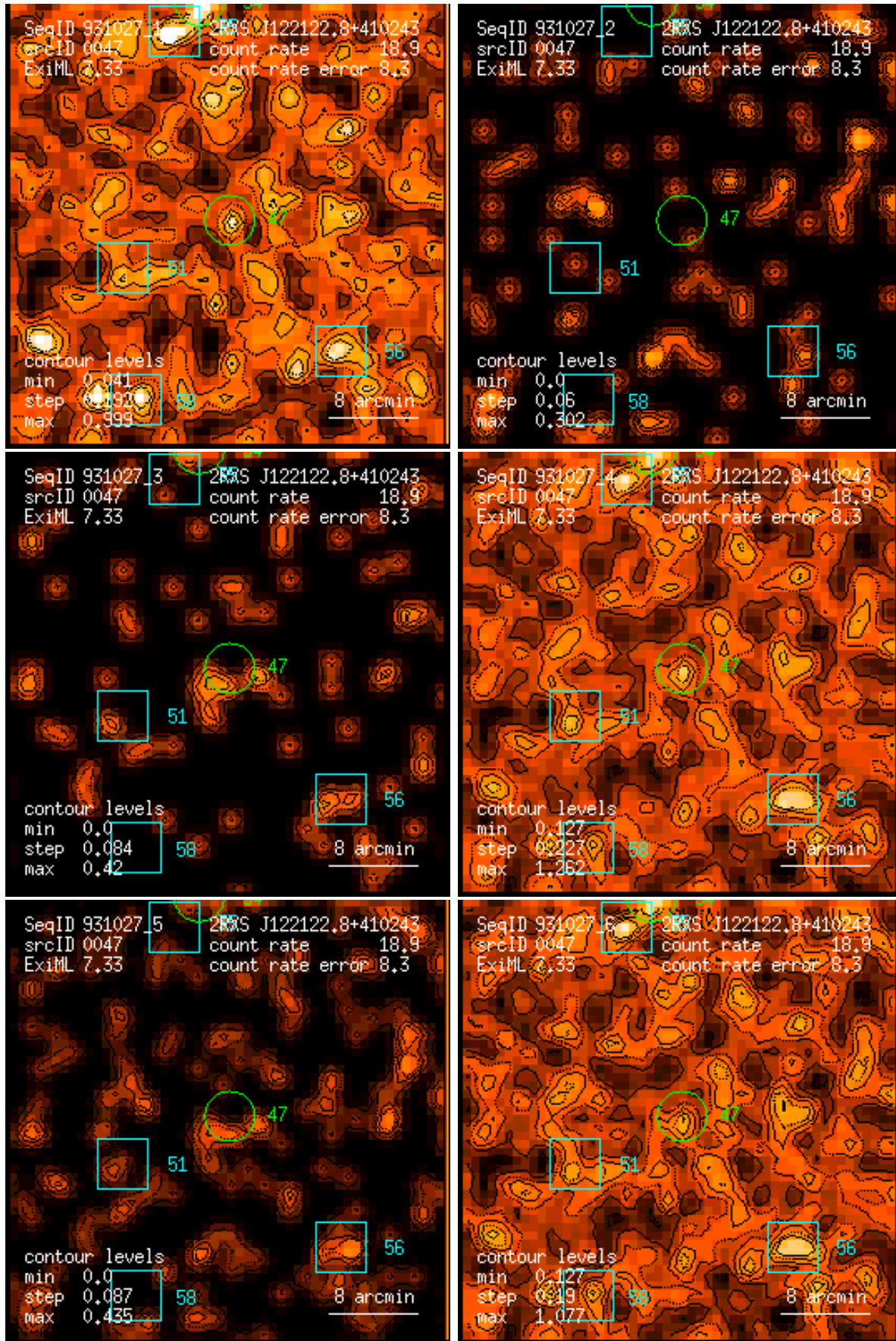
Figure 47: RASS 931027: detection 0047: band rate images, Gaussian filter: (1) PSPC channels 11 – 41, (2) 52 – 90, (3) 91 – 201, (4) 11 – 235, (5) 52 – 201, (6) 11 – 201. Broad band rates in counts/ks. Band rate contour levels in counts/ks/arcmin 2 .
