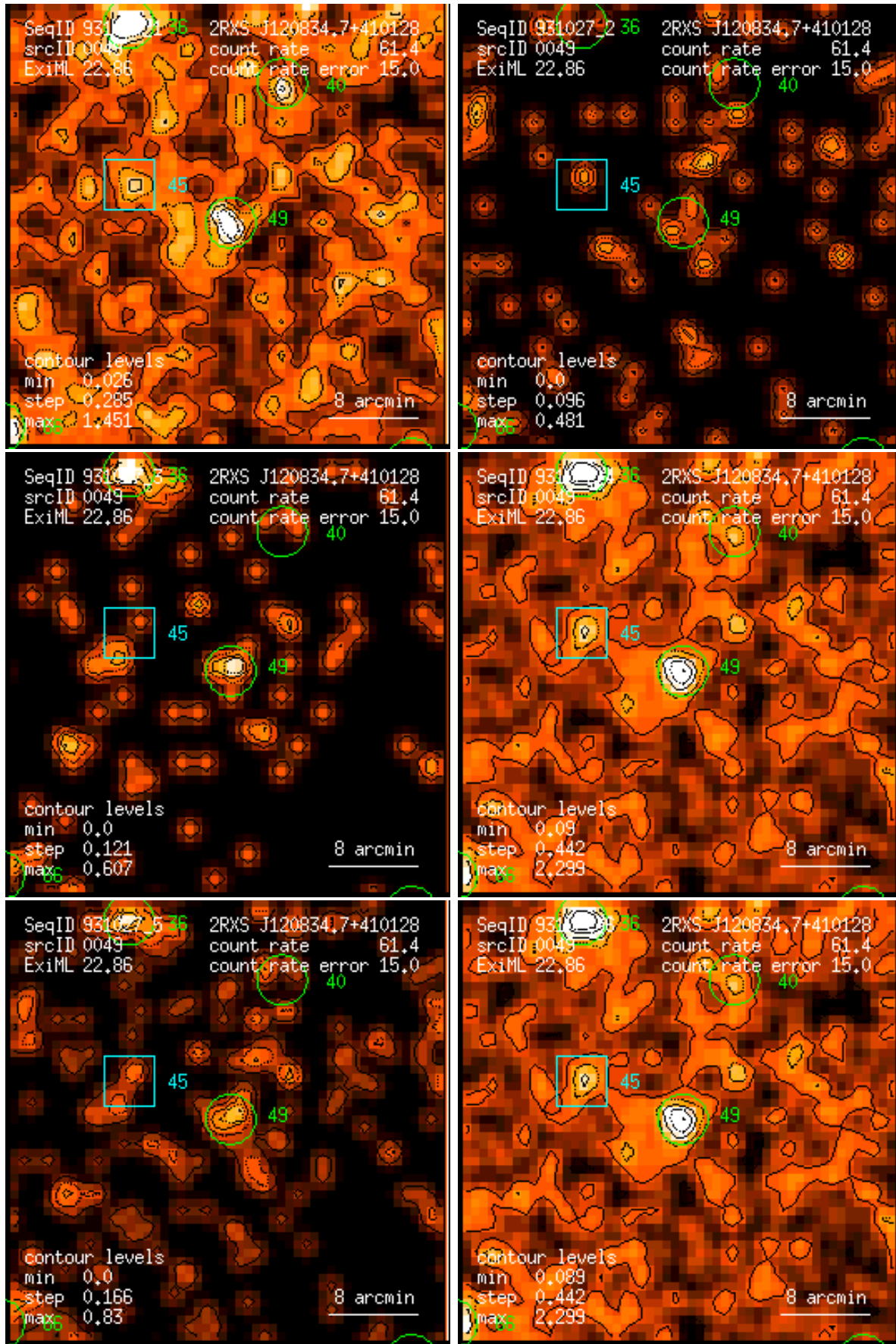
Figure 49: RASS 931027: detection 0049: band rate images, Gaussian filter: (1) PSPC channels 11 – 41, (2) 52 – 90, (3) 91 – 201, (4) 11 – 235, (5) 52 – 201, (6) 11 – 201. Broad band rates in counts/ks. Band rate contour levels in counts/ks/arcmin 2 .
