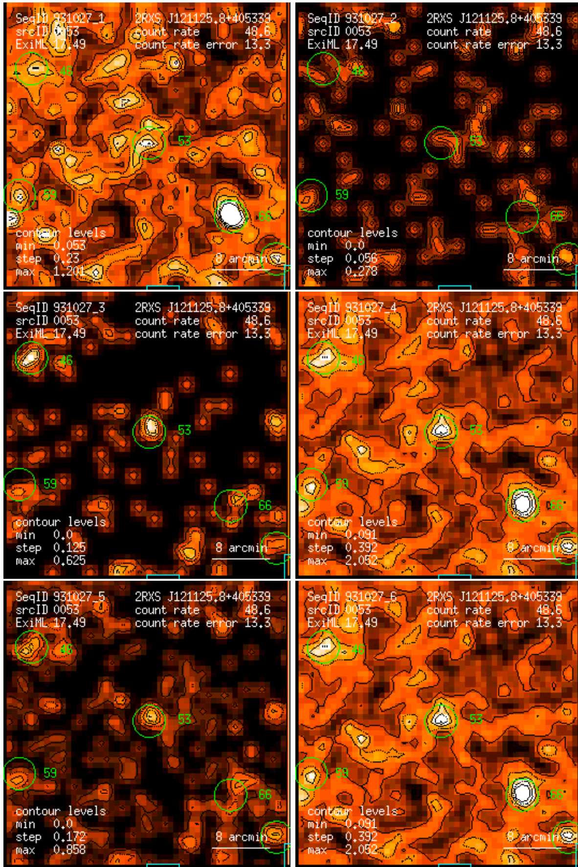
Figure 53: RASS 931027: detection 0053: band rate images, Gaussian filter: (1) PSPC channels 11 – 41, (2) 52 – 90, (3) 91 – 201, (4) 11 – 235, (5) 52 – 201, (6) 11 – 201. Broad band rates in counts/ks. Band rate contour levels in counts/ks/arcmin 2 .
