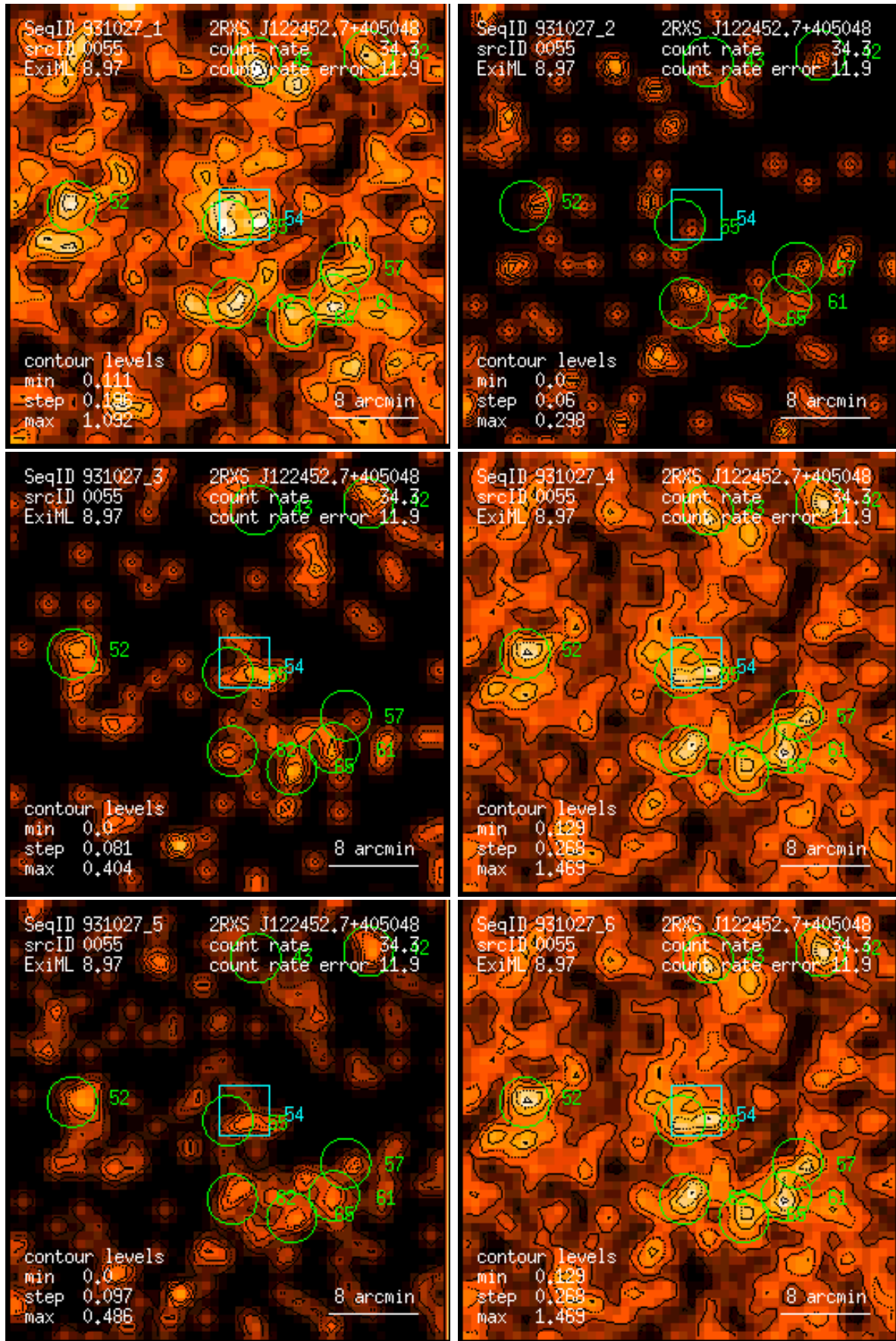
Figure 55: RASS 931027: detection 0055: band rate images, Gaussian filter: (1) PSPC channels 11 – 41, (2) 52 – 90, (3) 91 – 201, (4) 11 – 235, (5) 52 – 201, (6) 11 – 201. Broad band rates in counts/ks. Band rate contour levels in counts/ks/arcmin 2 .
