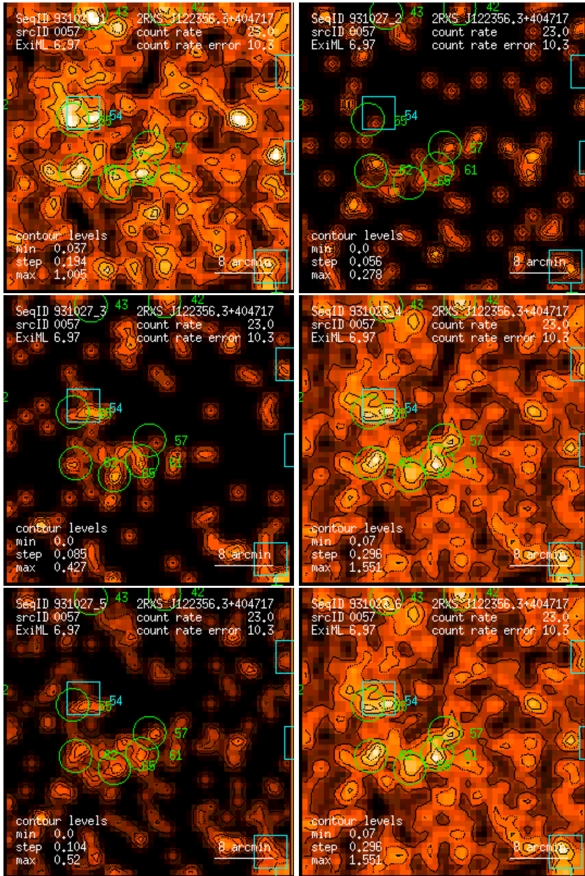
Figure 57: RASS 931027: detection 0057: band rate images, Gaussian filter: (1) PSPC channels 11 – 41, (2) 52 – 90, (3) 91 – 201, (4) 11 – 235, (5) 52 – 201, (6) 11 – 201. Broad band rates in counts/ks. Band rate contour levels in counts/ks/arcmin 2 .
