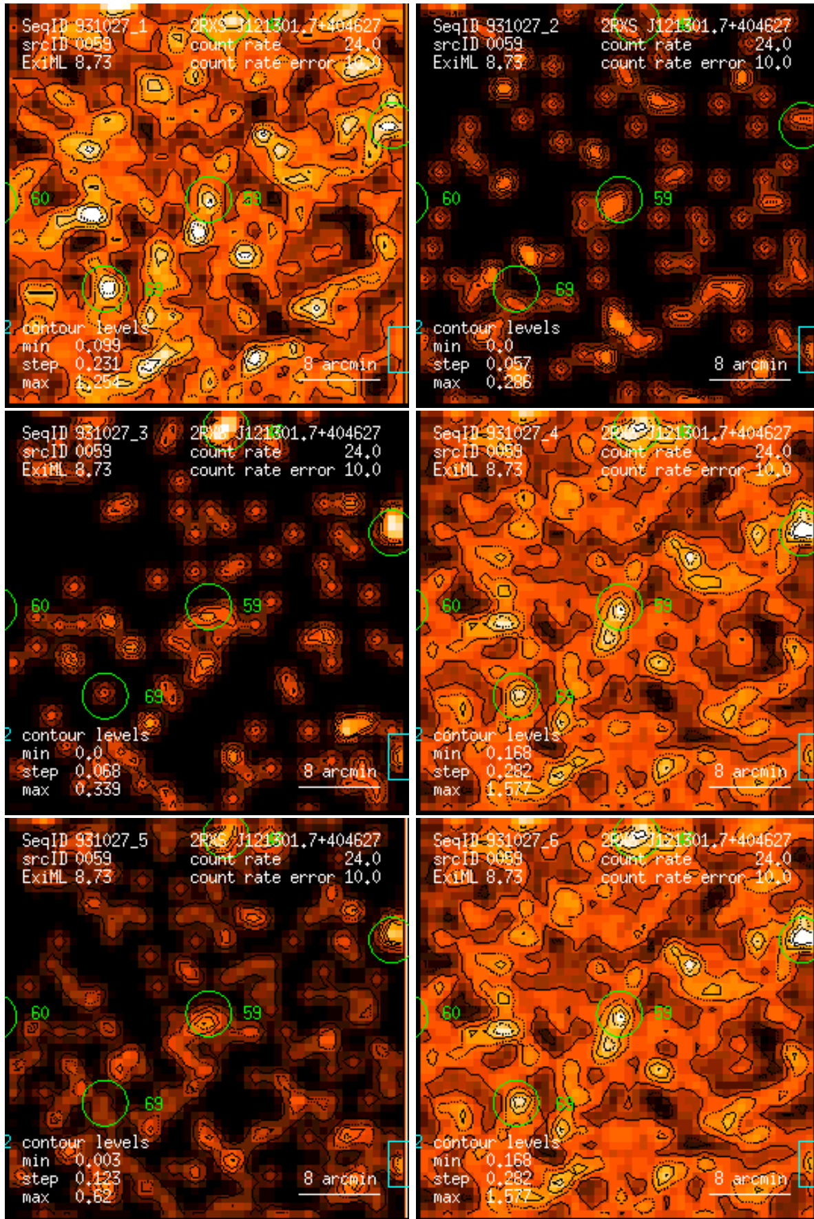
Figure 59: RASS 931027: detection 0059: band rate images, Gaussian filter: (1) PSPC channels 11 – 41, (2) 52 – 90, (3) 91 – 201, (4) 11 – 235, (5) 52 – 201, (6) 11 – 201. Broad band rates in counts/ks. Band rate contour levels in counts/ks/arcmin 2 .
