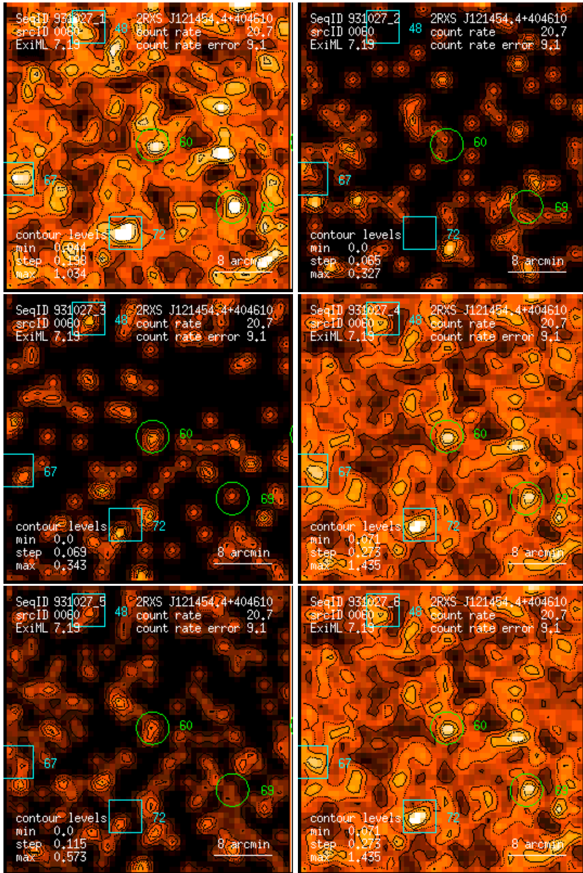
Figure 60: RASS 931027: detection 0060: band rate images, Gaussian filter: (1) PSPC channels 11 – 41, (2) 52 – 90, (3) 91 – 201, (4) 11 – 235, (5) 52 – 201, (6) 11 – 201. Broad band rates in counts/ks. Band rate contour levels in counts/ks/arcmin 2 .
