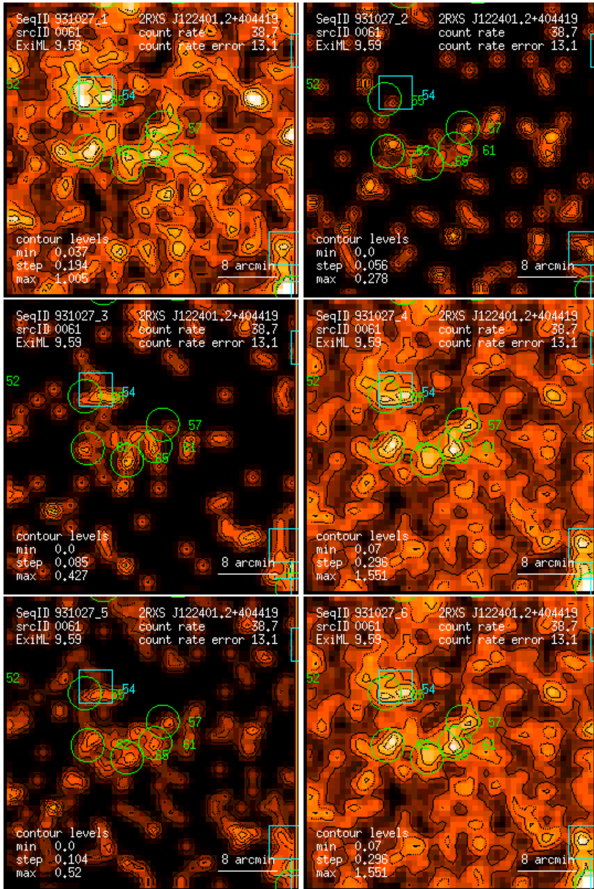
Figure 61: RASS 931027: detection 0061: band rate images, Gaussian filter: (1) PSPC channels 11 – 41, (2) 52 – 90, (3) 91 – 201, (4) 11 – 235, (5) 52 – 201, (6) 11 – 201. Broad band rates in counts/ks. Band rate contour levels in counts/ks/arcmin 2 .
