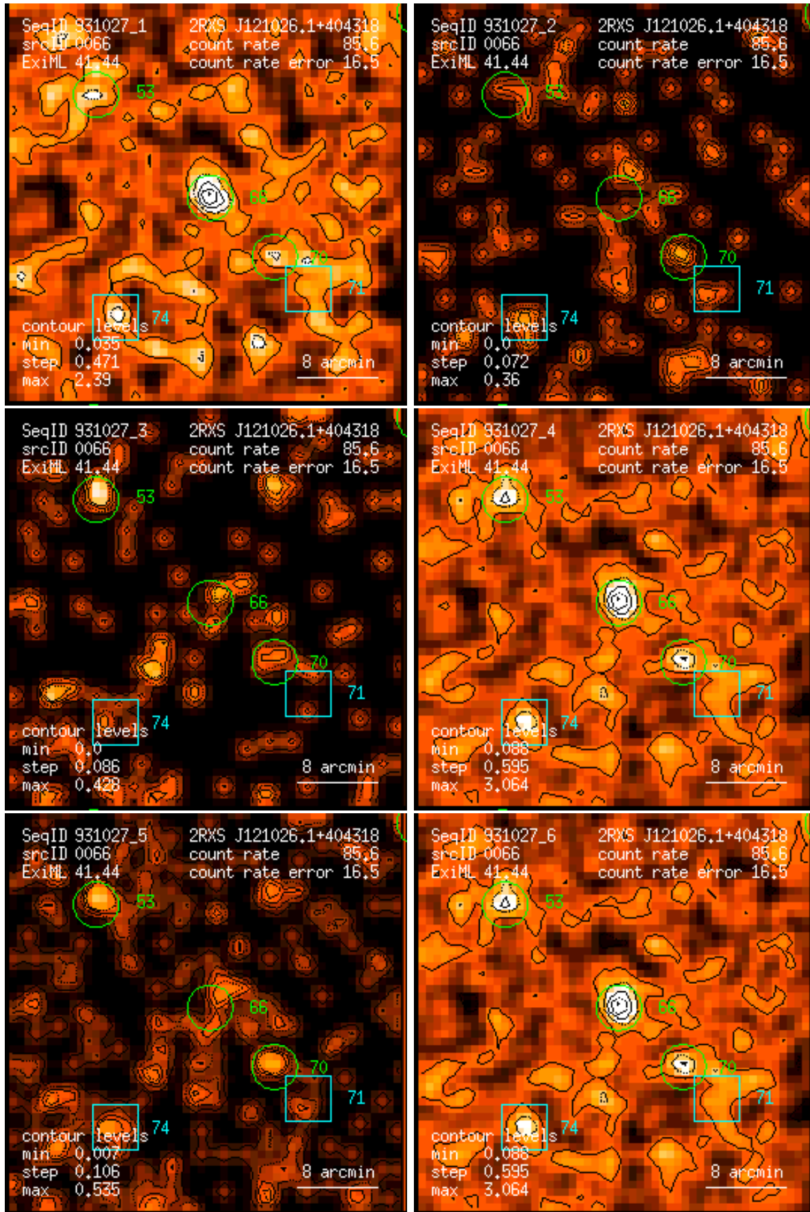
Figure 66: RASS 931027: detection 0066: band rate images, Gaussian filter: (1) PSPC channels 11 – 41, (2) 52 – 90, (3) 91 – 201, (4) 11 – 235, (5) 52 – 201, (6) 11 – 201. Broad band rates in counts/ks. Band rate contour levels in counts/ks/arcmin 2 .
