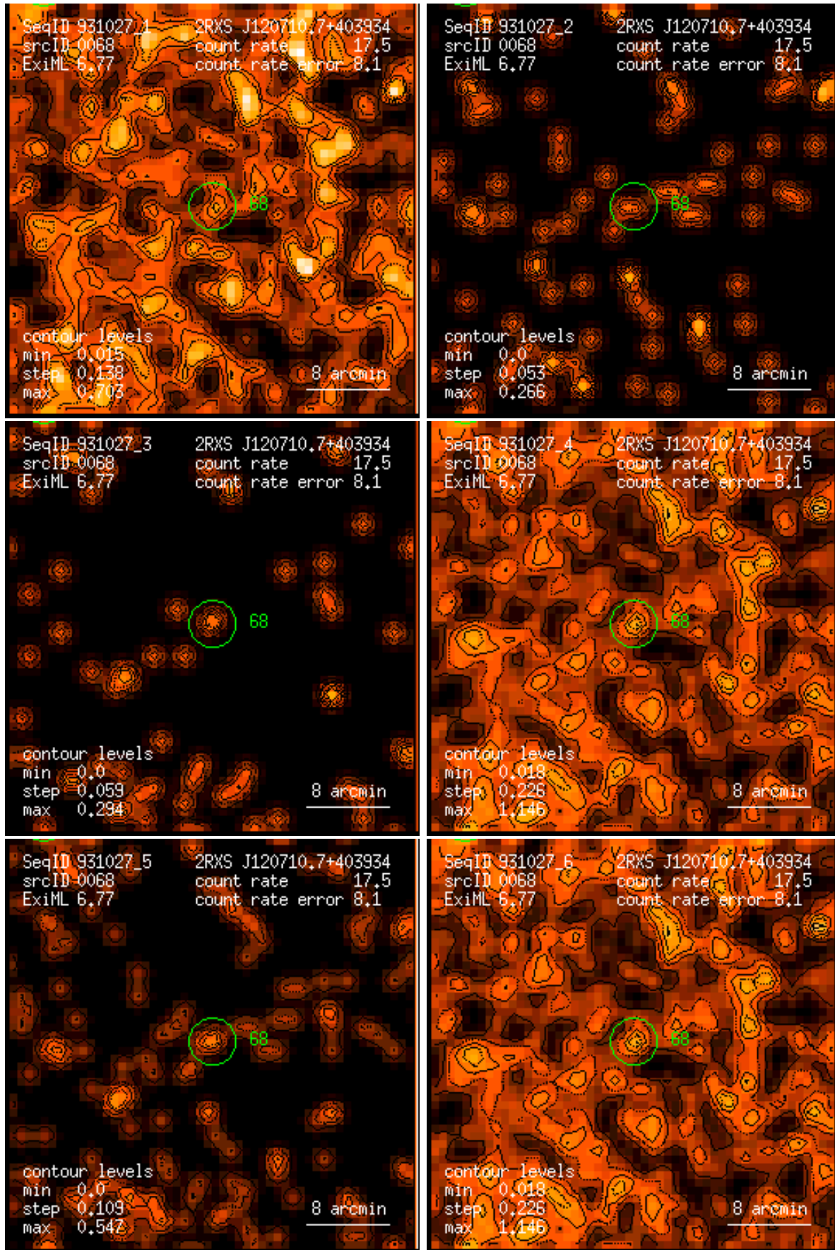
Figure 68: RASS 931027: detection 0068: band rate images, Gaussian filter: (1) PSPC channels 11 – 41, (2) 52 – 90, (3) 91 – 201, (4) 11 – 235, (5) 52 – 201, (6) 11 – 201. Broad band rates in counts/ks. Band rate contour levels in counts/ks/arcmin 2 .
