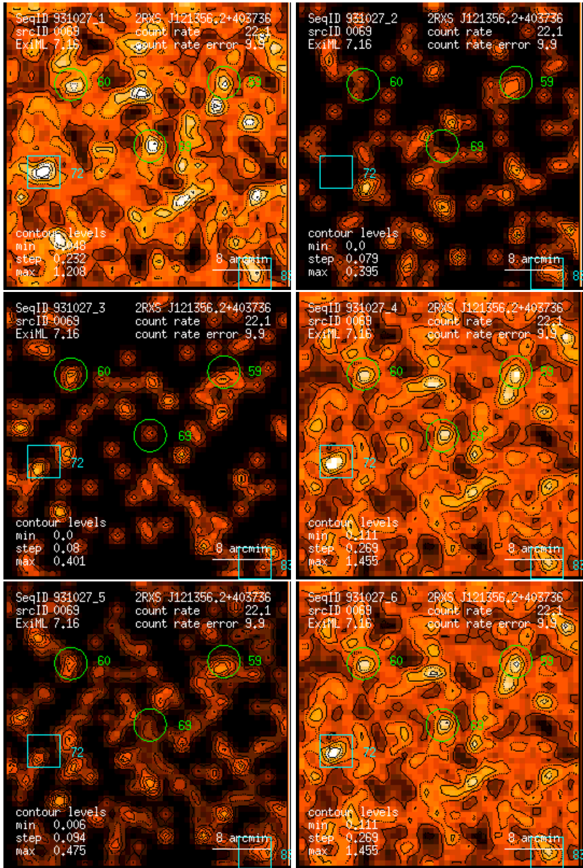
Figure 69: RASS 931027: detection 0069: band rate images, Gaussian filter: (1) PSPC channels 11 – 41, (2) 52 – 90, (3) 91 – 201, (4) 11 – 235, (5) 52 – 201, (6) 11 – 201. Broad band rates in counts/ks. Band rate contour levels in counts/ks/arcmin 2 .
